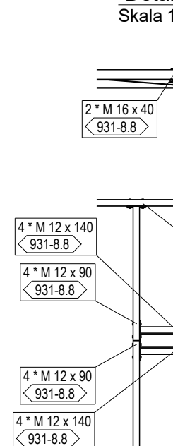
Detail F Skala 1:50
