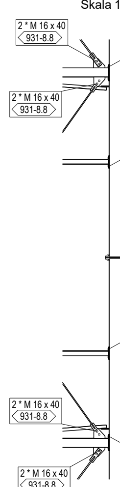
Detail G Skala 1:50
