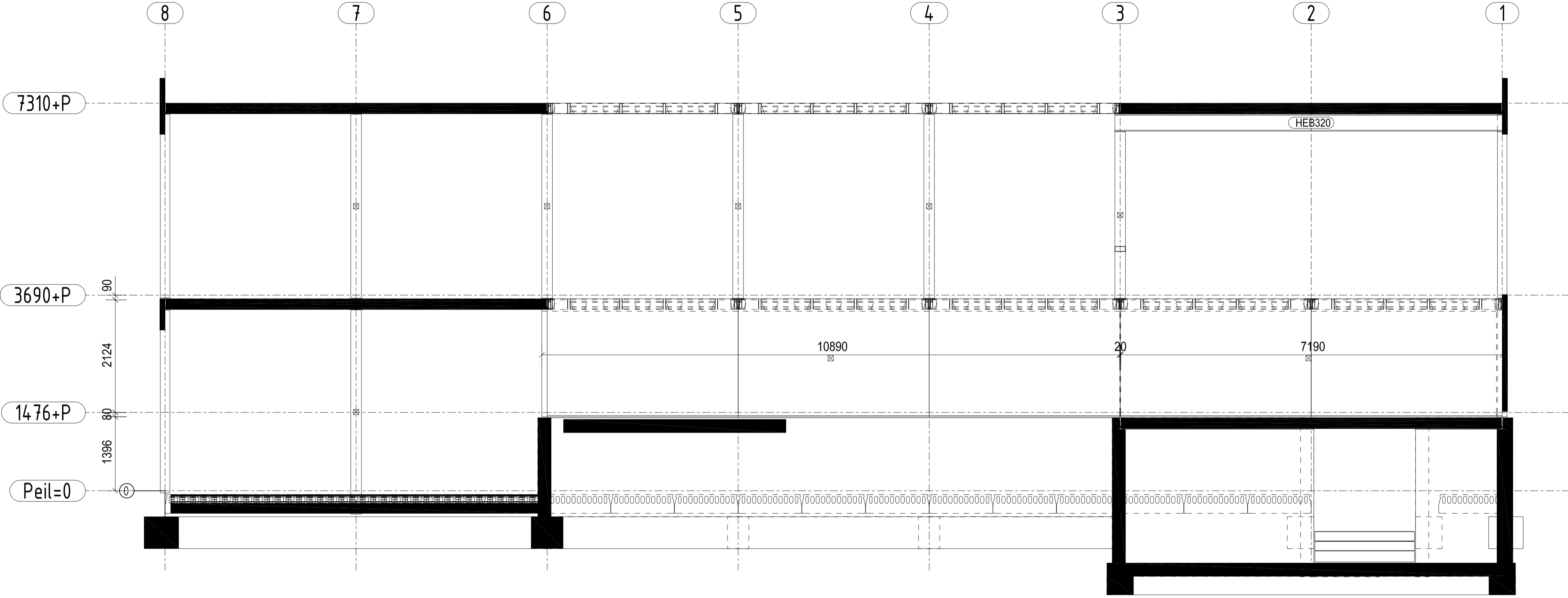
WANDAANZICHT AS E 1:50
