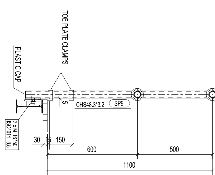
STANDARD POST - STAIRS TYPICAL DETAIL
