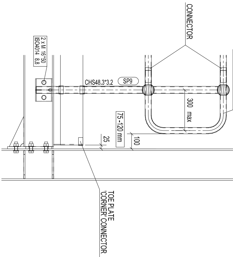
STANDARD POST - PLATFORM TYPICAL DETAIL
