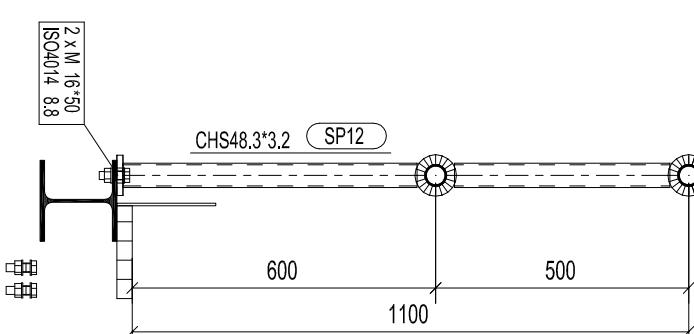
STANDARD POST - PLATFORM TYPICAL DETAIL
