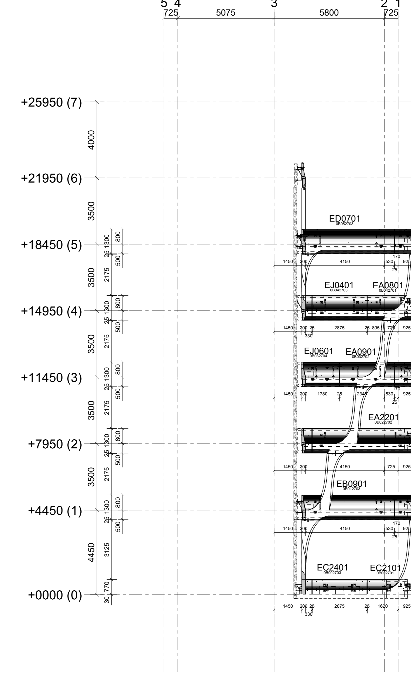
Achse C3
