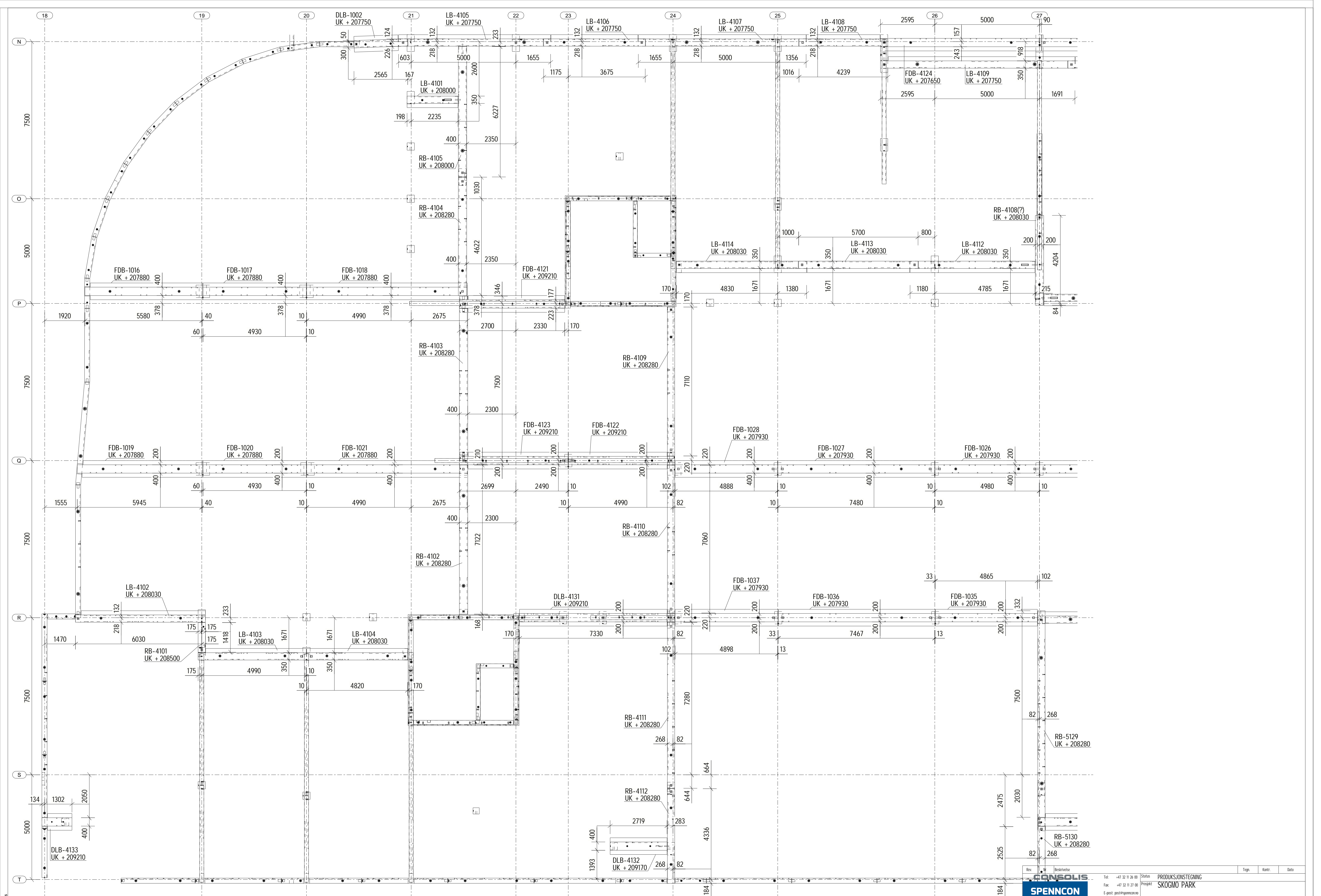
Plan 01_BJELKEPLAN 1:75
