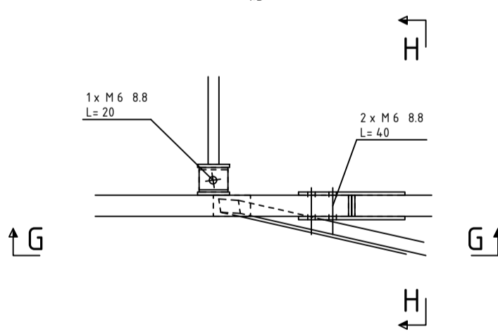
TOP VIEW 1:5
