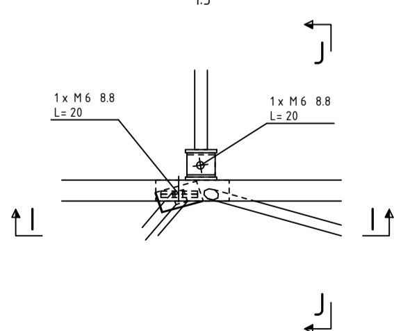
TOP VIEW 1:5
