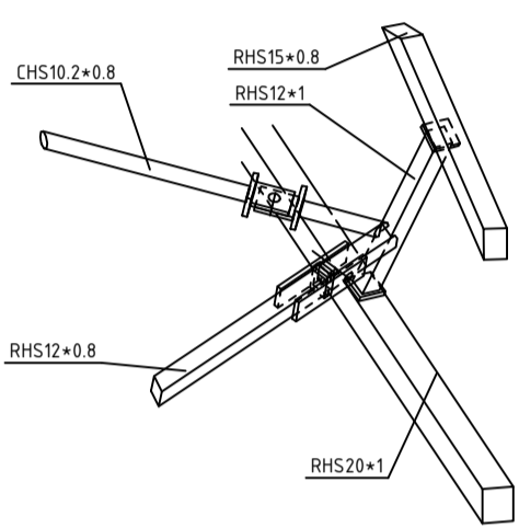
ISOMETRIC VIEW 1:5
