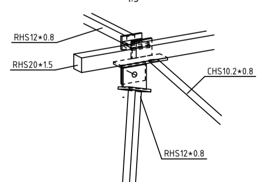
ISOMETRIC VIEW 1:5
