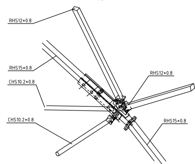
ISOMETRIC VIEW 1:5
