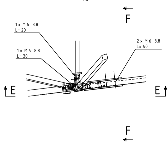
TOP VIEW 1:5
