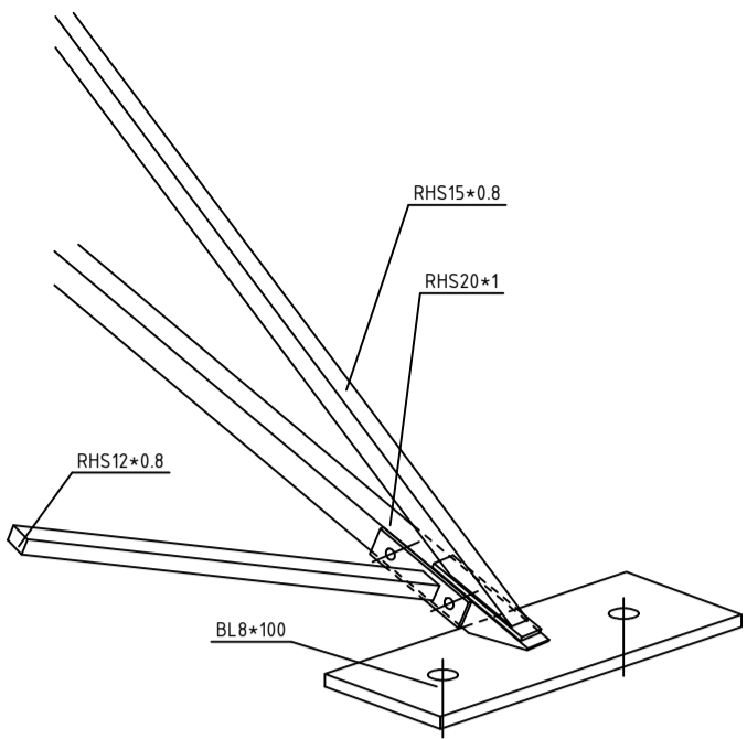
ISOMETRIC VIEW 1:5
