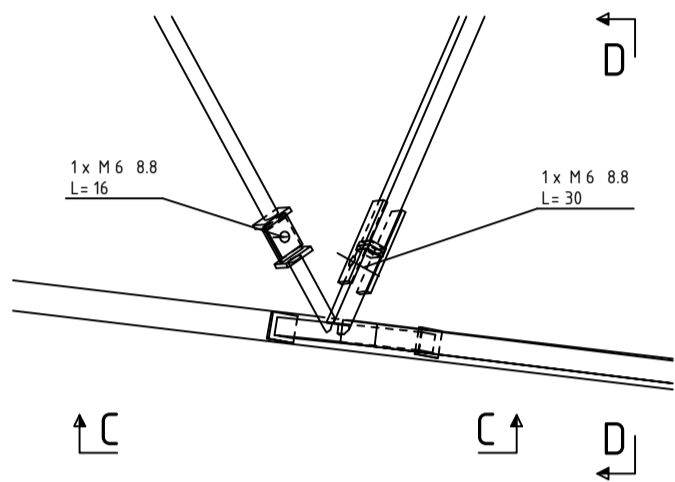
TOP VIEW 1:5
