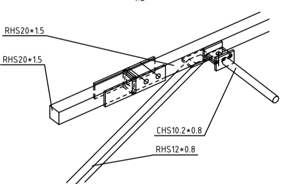
ISOMETRIC VIEW 1:5
