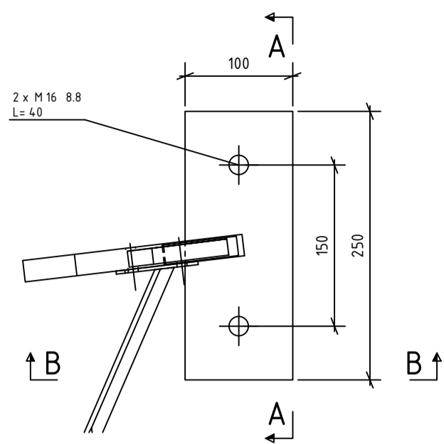
TOP VIEW 1:5
