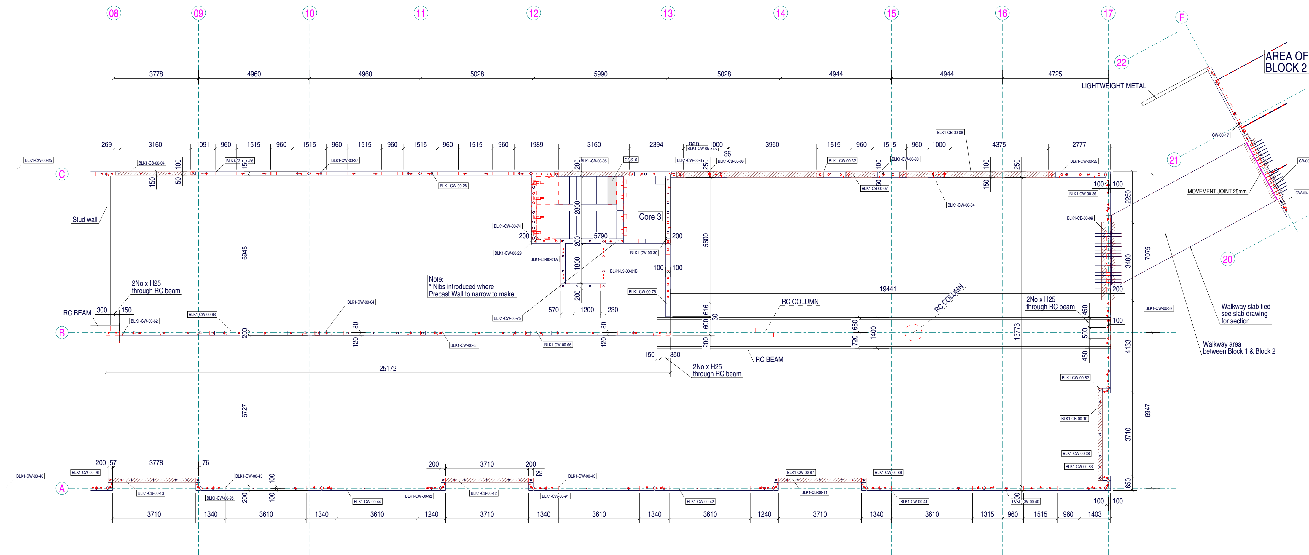
Wall layout 1:100
