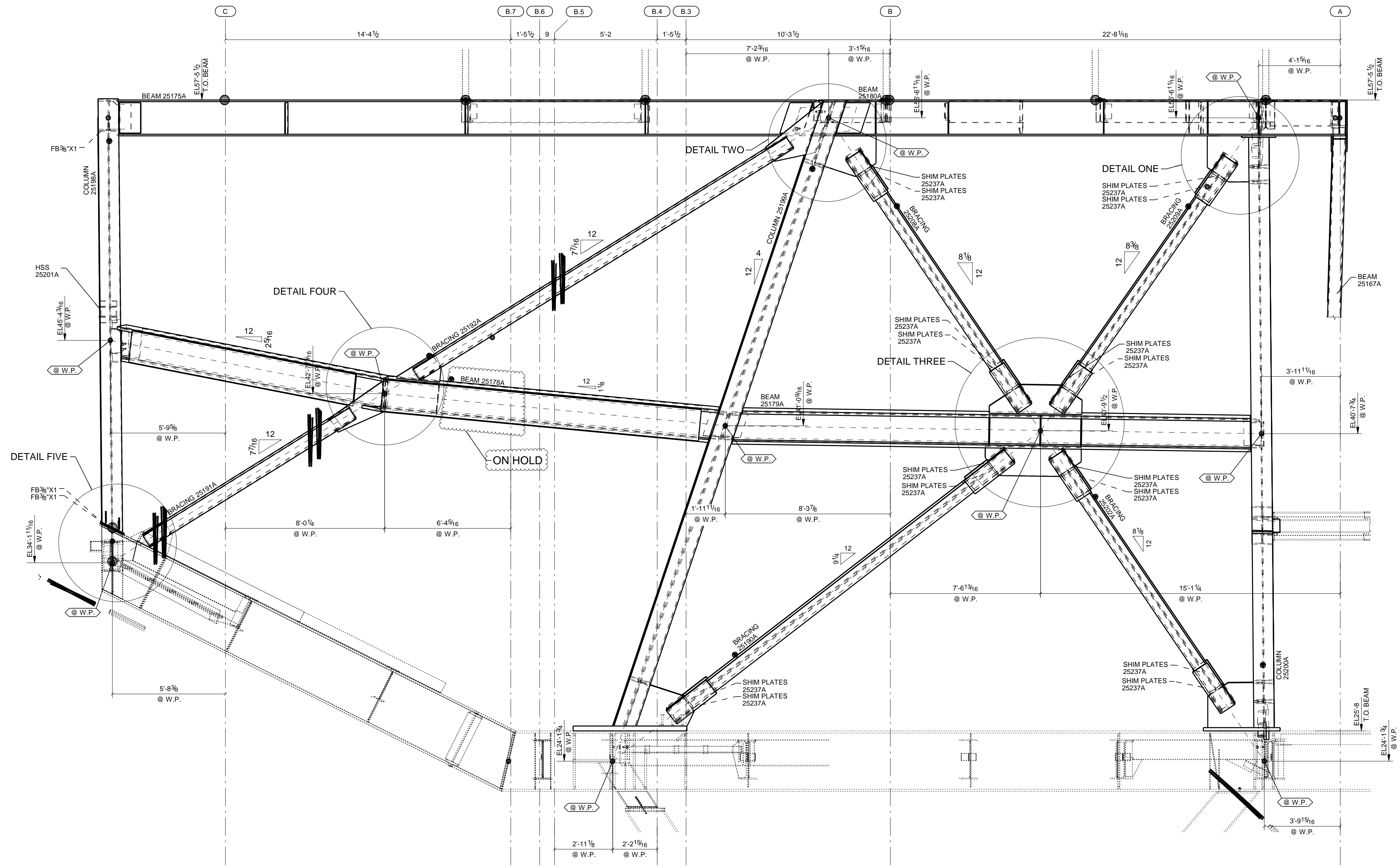
4/E293, 4/E294, 4/E295 ELEVATION VIEW CLASSROOM - NORTH FRAME ELEVATION (REF.: A/S-502)
