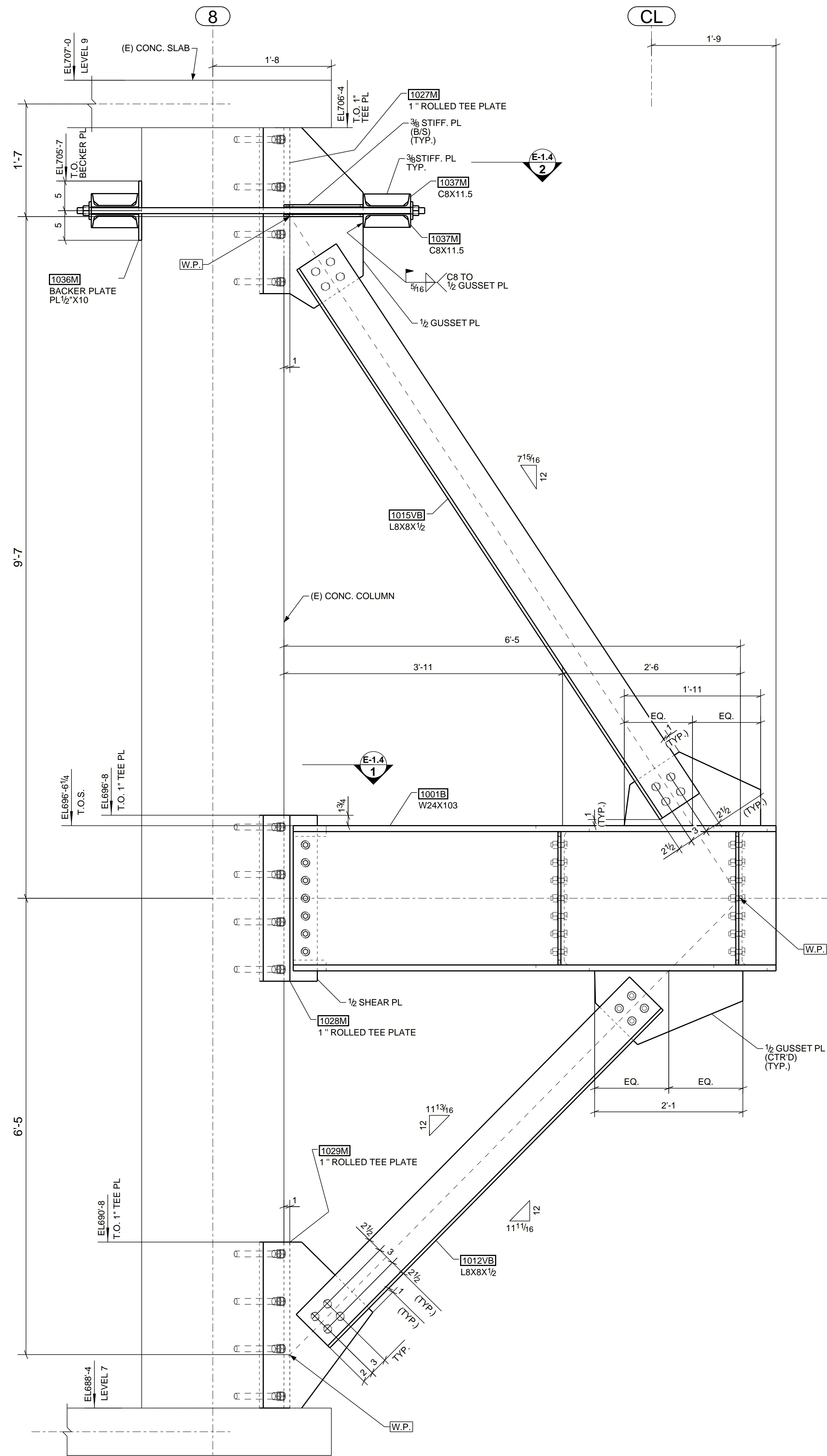
A STEEL BRACKET @ ROUND COLUMN REF.: 6 / MC-5
