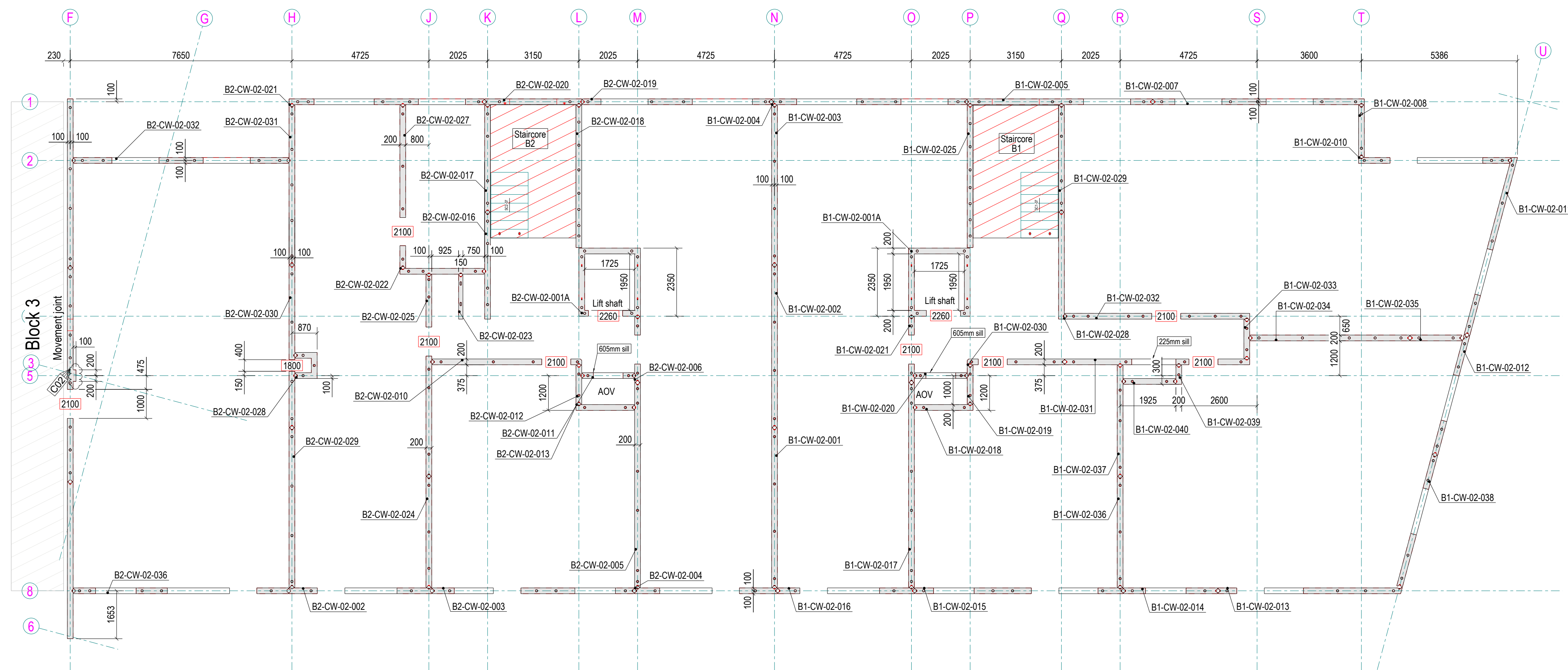
Block 1 and 2: Second floor wall layout @ +81.575 1:100
