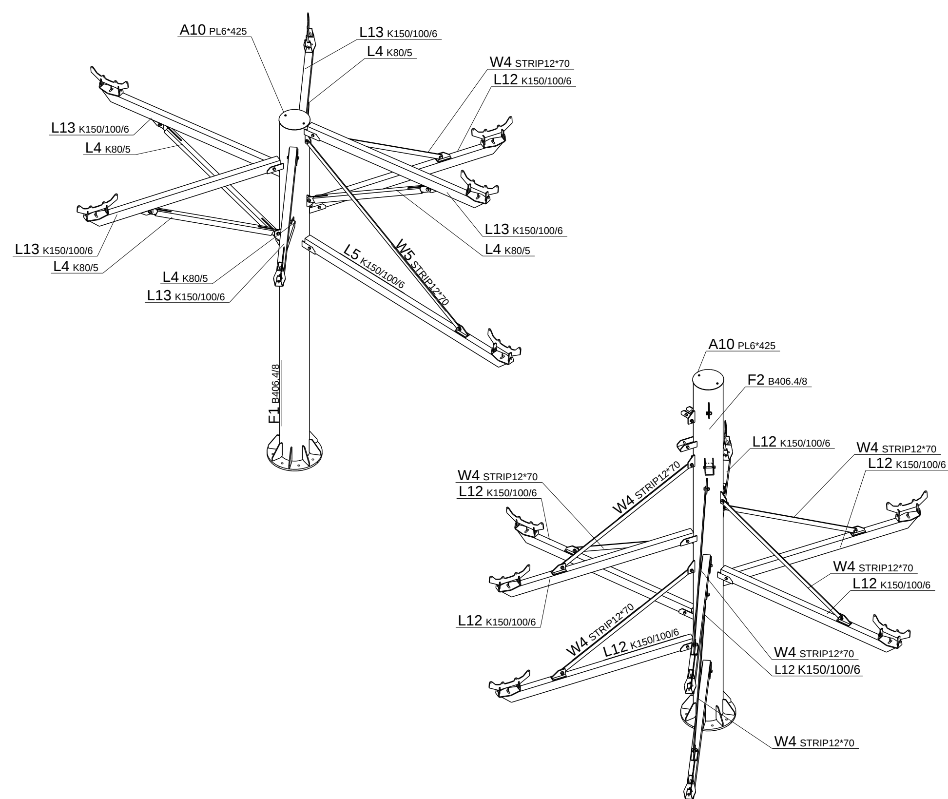
dsn 3D - 3D, 1:50
