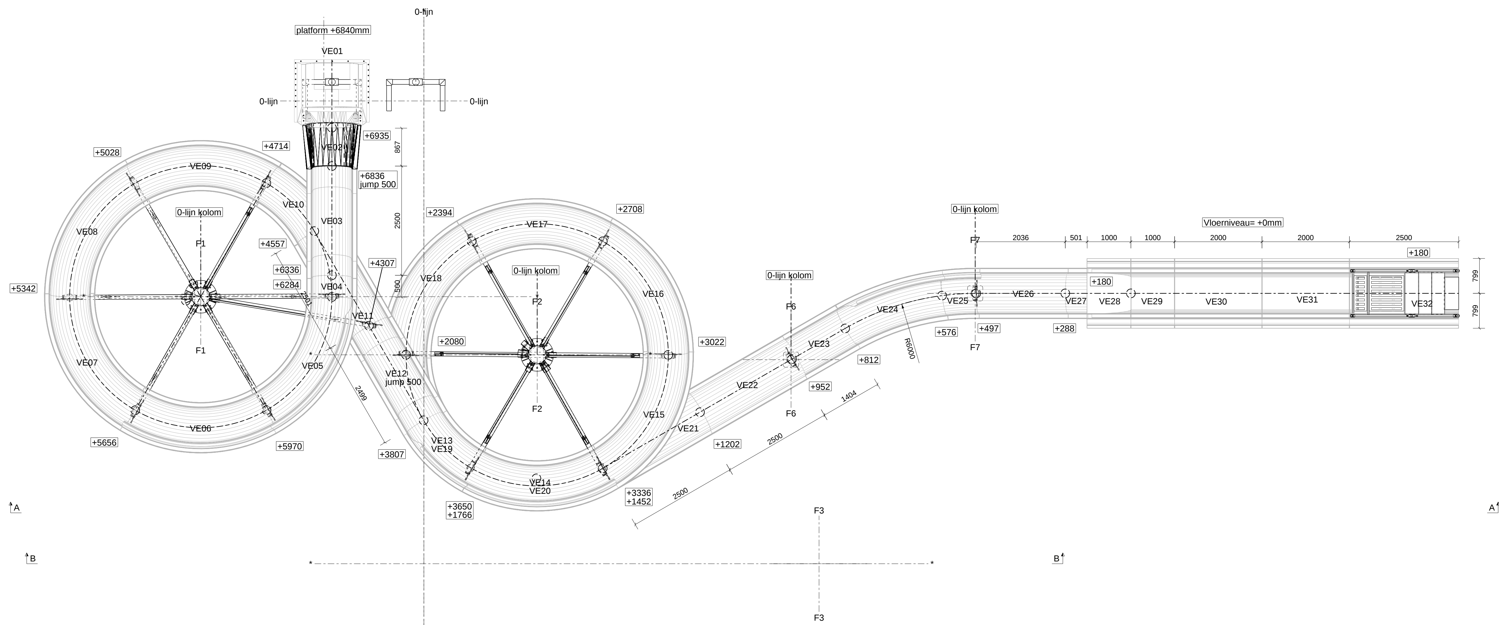
dsn 3D - 3D, 1:50
