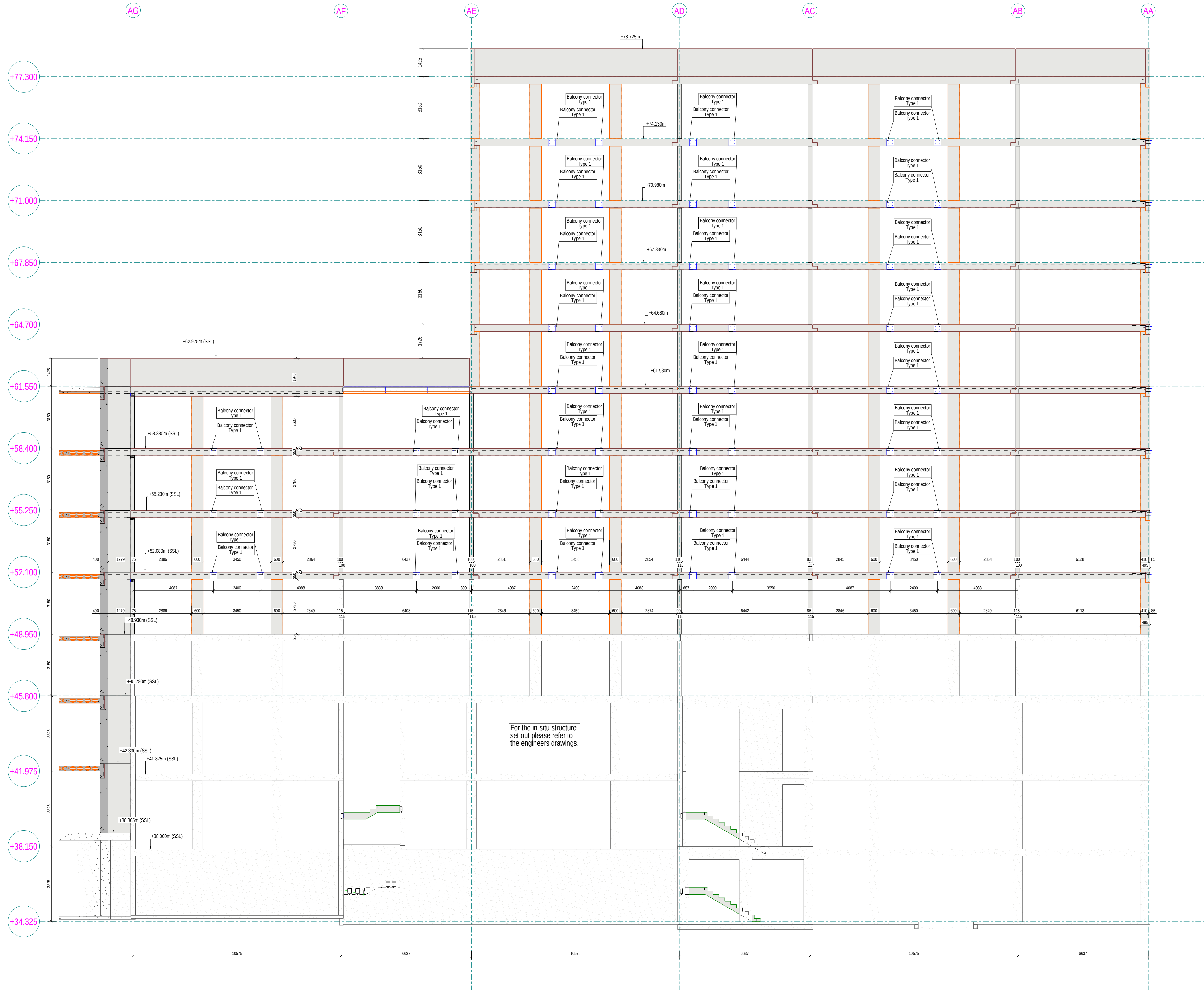
Section 6 - 6 Elevation GL/A4
