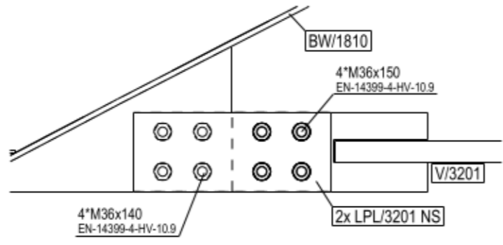
DETAIL C 1:20
