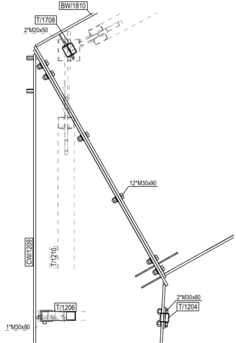
DETAIL A 1:20
