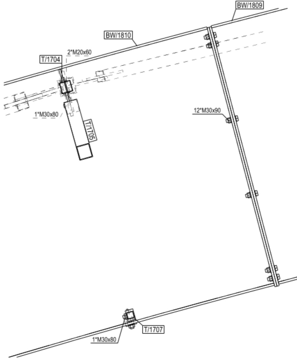
DETAIL D 1:20
