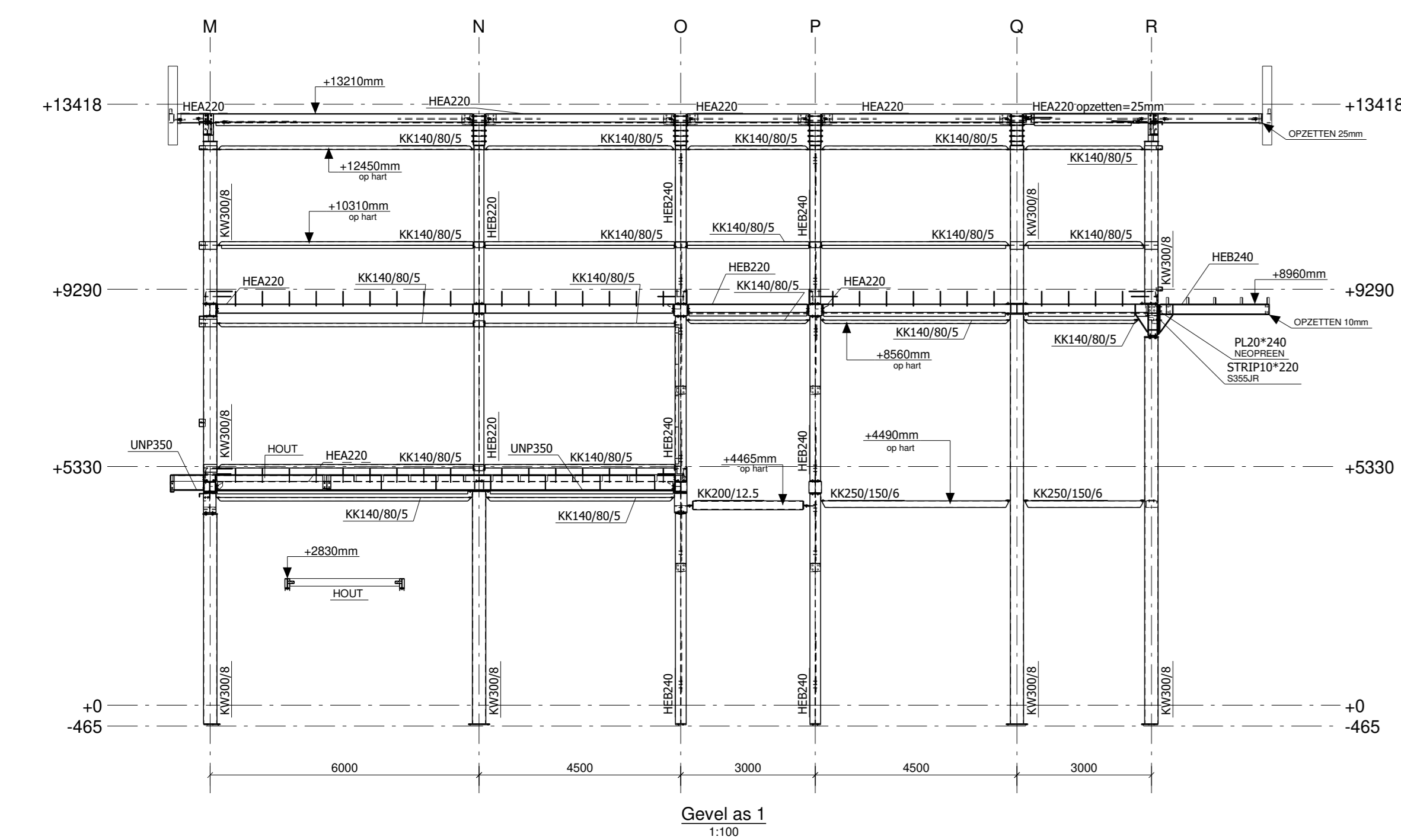
Gevel as 1 1:100
