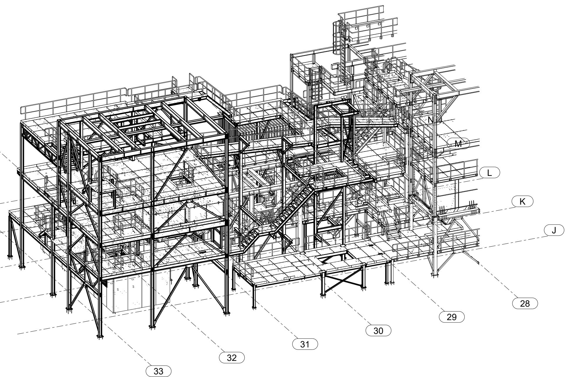
CRUSHER AREA - AXONOMETRY 1:150
