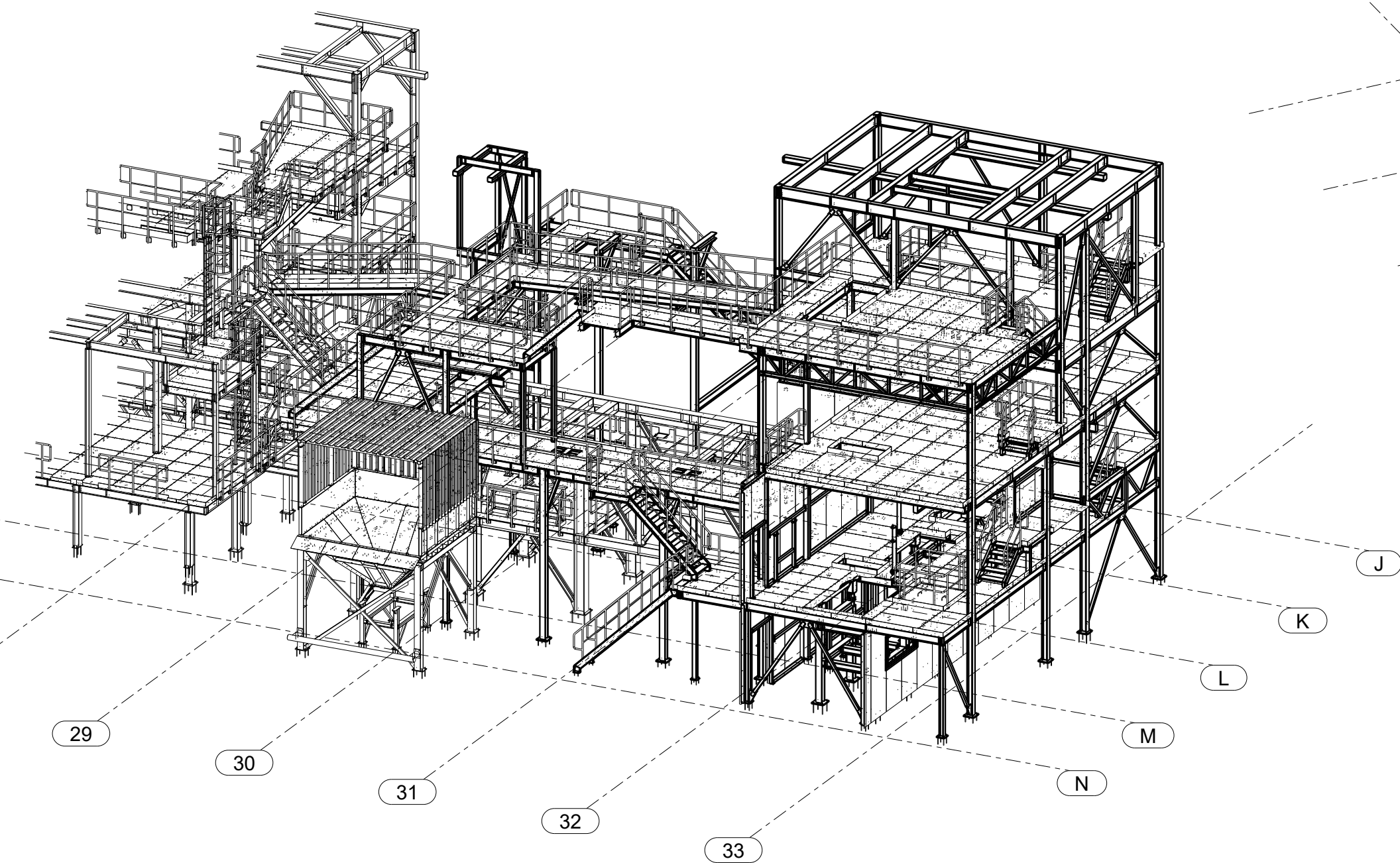
CRUSHER AREA - AXONOMETRY 1:150
