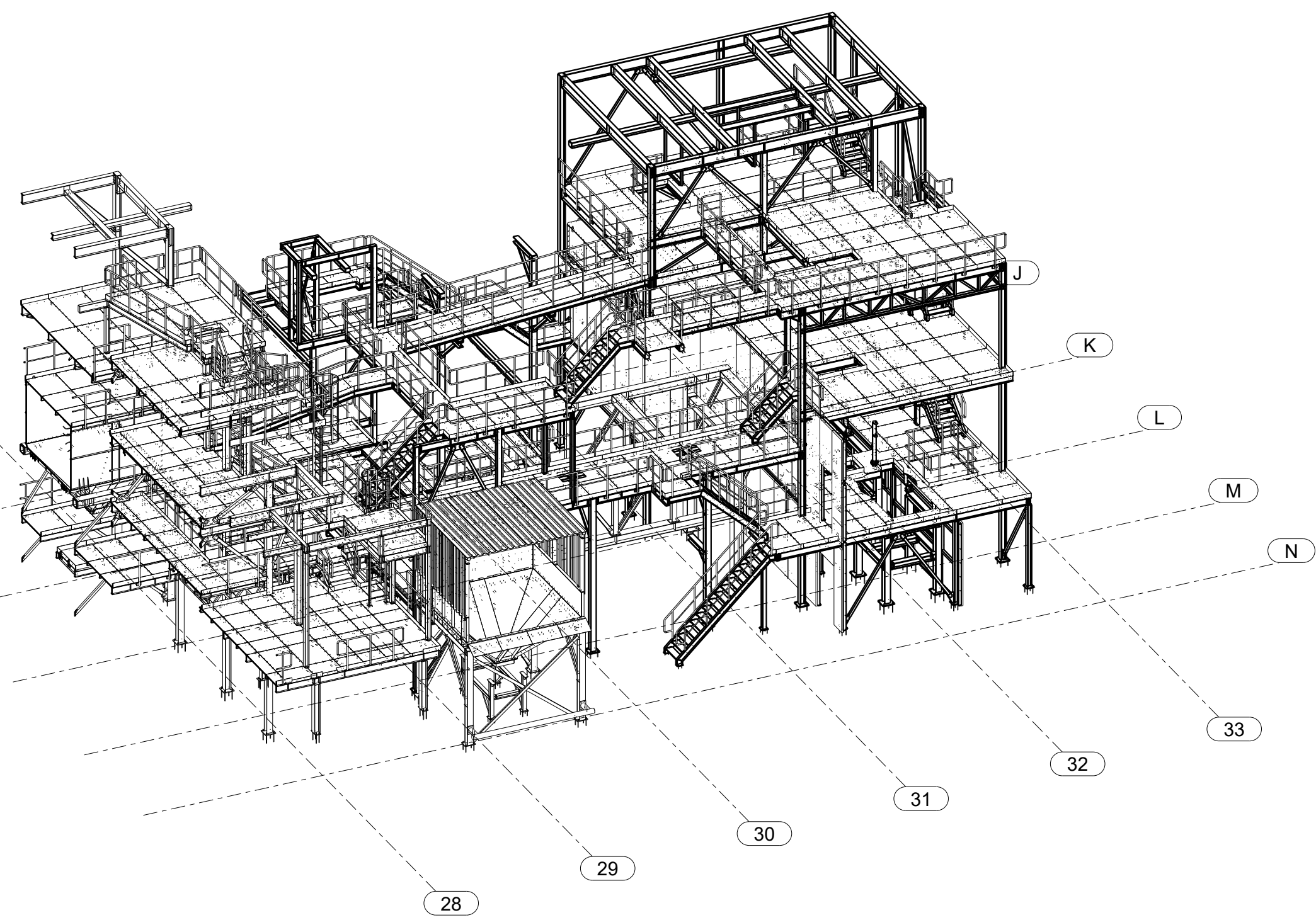
CRUSHER AREA - AXONOMETRY 1:150
