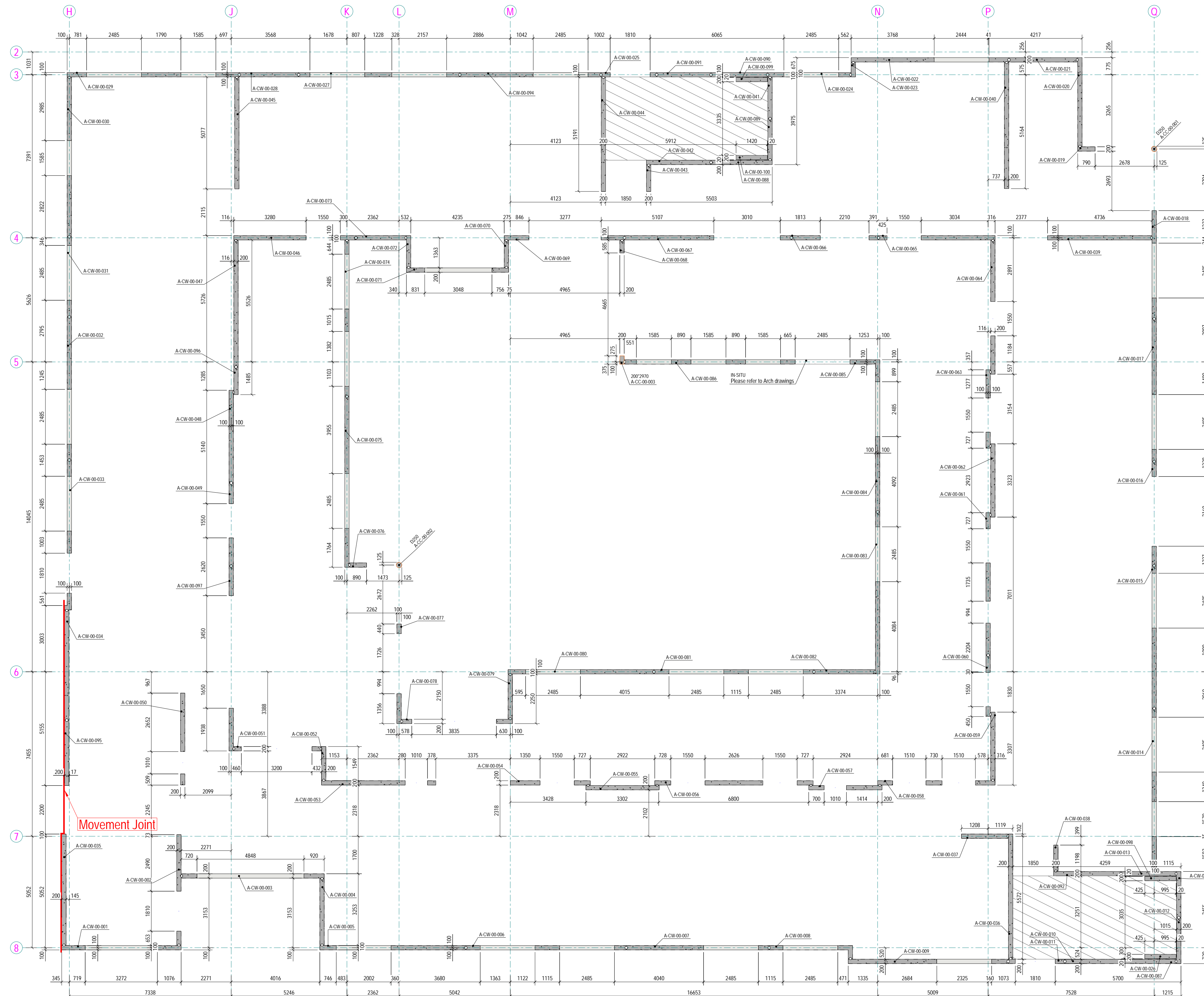
Block A: Ground Floor Wall Layout 1:100
