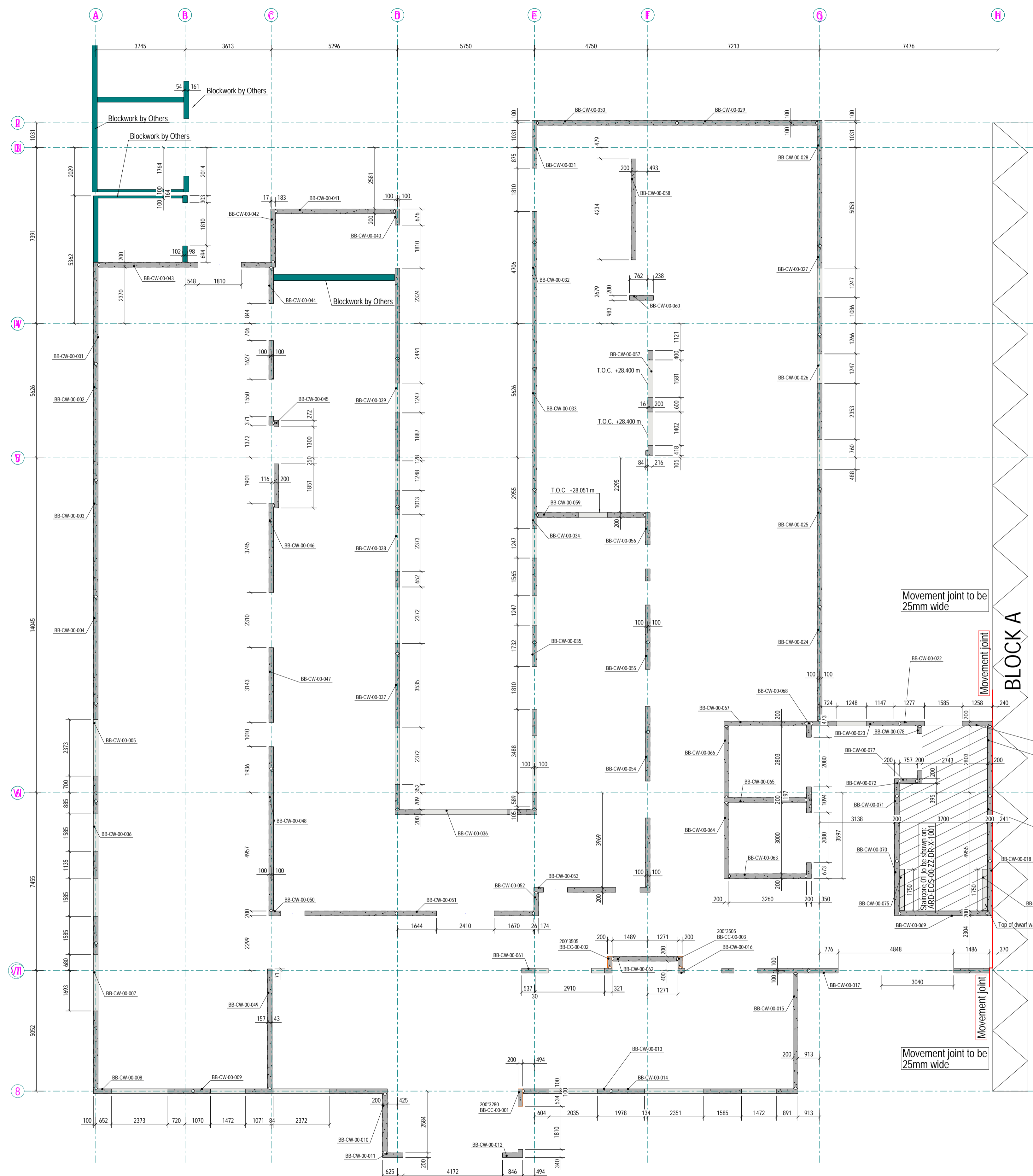
Block B: Ground Floor Wall Layout 1:100
