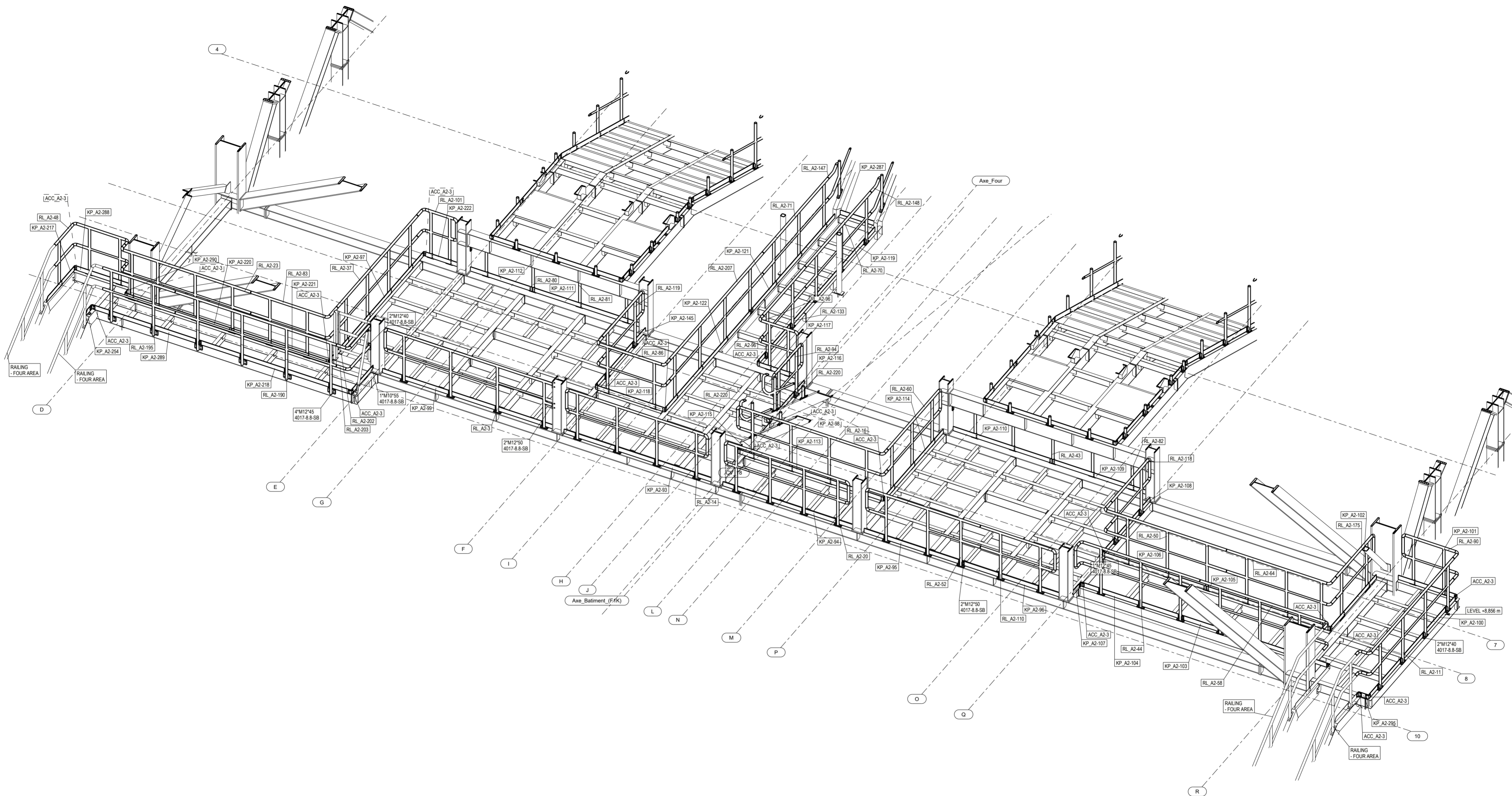
RAILINGS - LEVEL +8.856m 1:50
