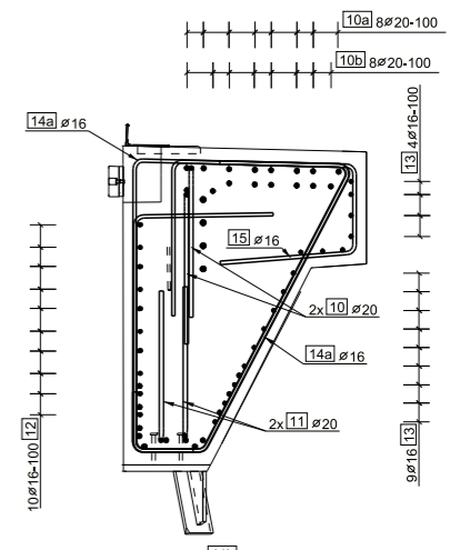
Section F - F BEFORE RHS PIPE 1:20
