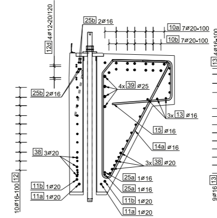
Section E - E THROUGH RHS PIPE 1:20
