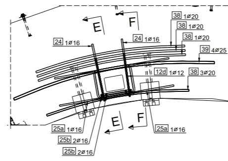
Detail 2 SUPPORT 1:20
