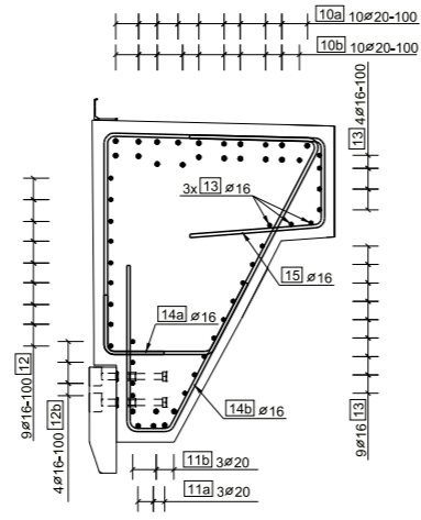
Detail 1.1 DUCTING HOLE 1:20
