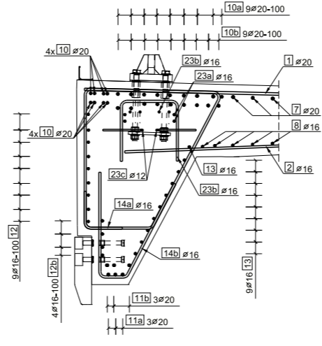
Section I - I LIFTING 1:20
