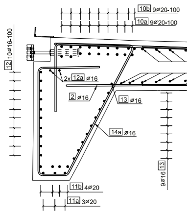
Section C - C JACK RECESS 1:20
