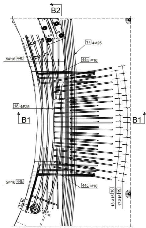
Detail 1.1 DUCTING HOLE 1:20
