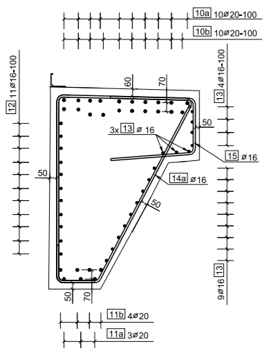
Section A - A GENERAL REINFORCEMENT RING BEAM 1:20
