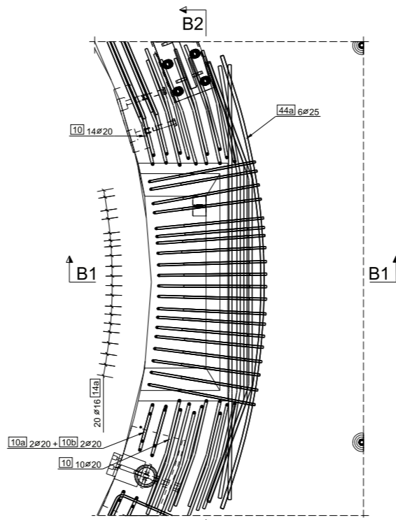
Detail 1.2 DUCTING HOLE 1:20
