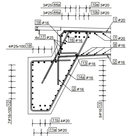
Section B1 - B1 1:20
