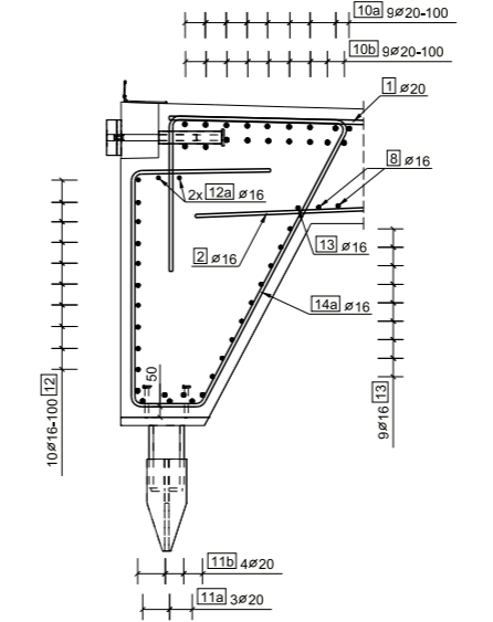
Section J - J LIFTING PIN 1:20
