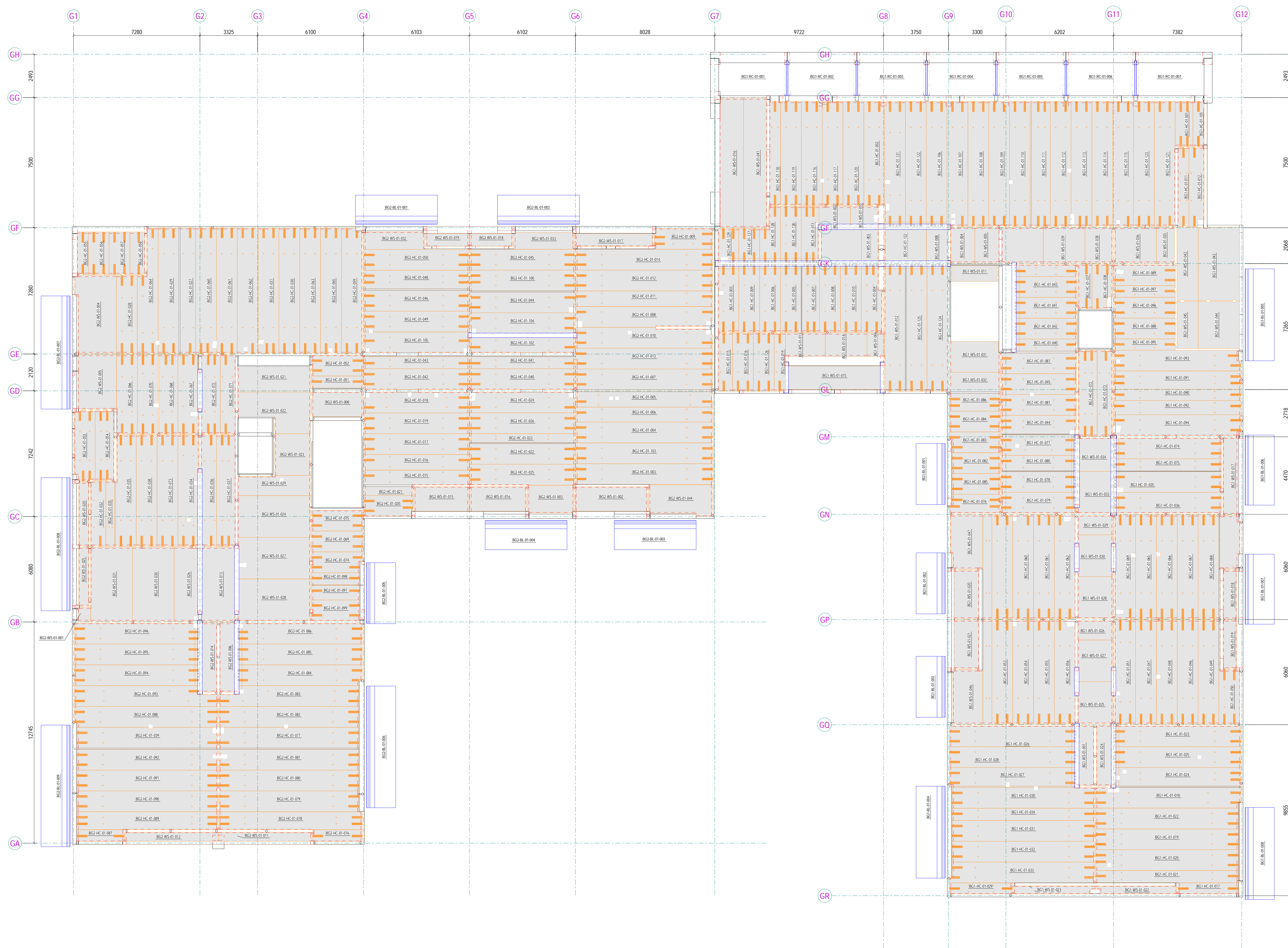
Block G: First Floor Wall Layout 1:100
