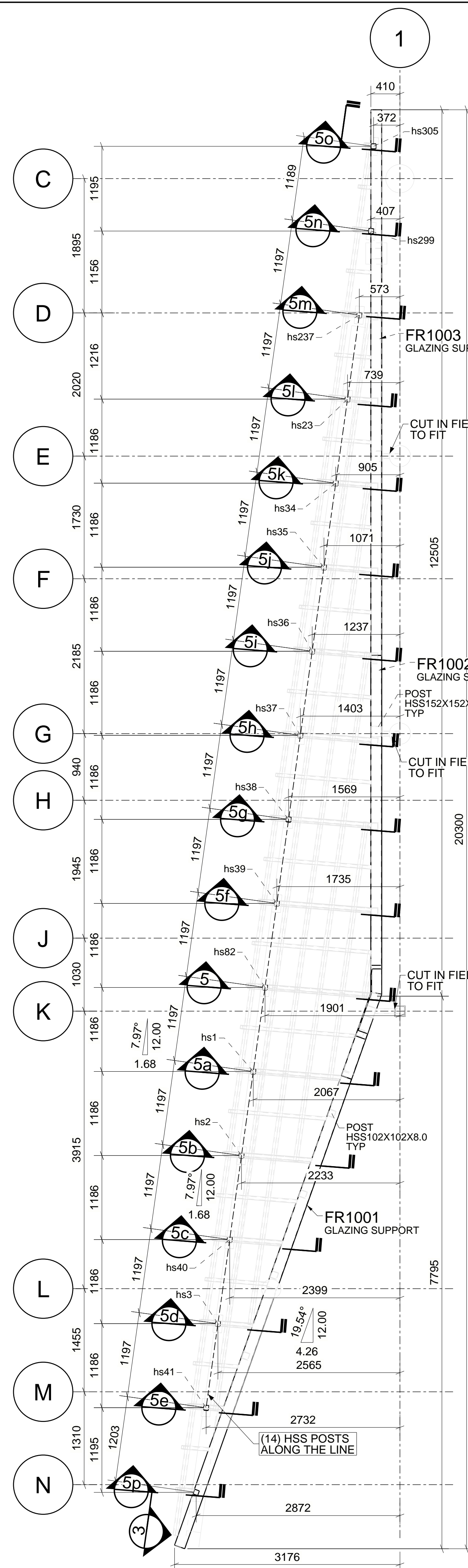
SLOPED MASONRY STEEL LAYOUT T.O.S. EL.: SEE PLAN REF.: 1/S411
