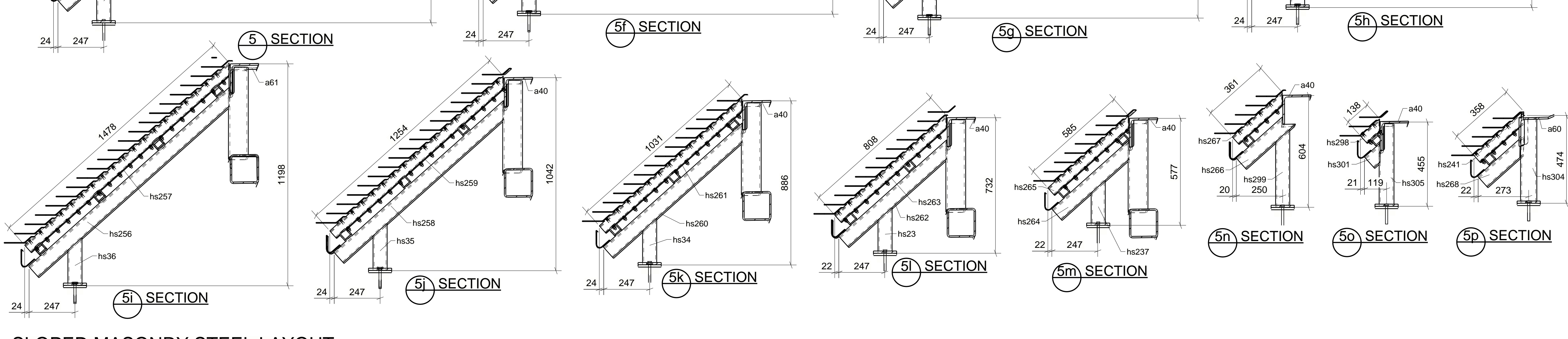
SLOPED MASONRY STEEL LAYOUT T.O.S. EL.: SEE PLAN REF.: 1/S411
