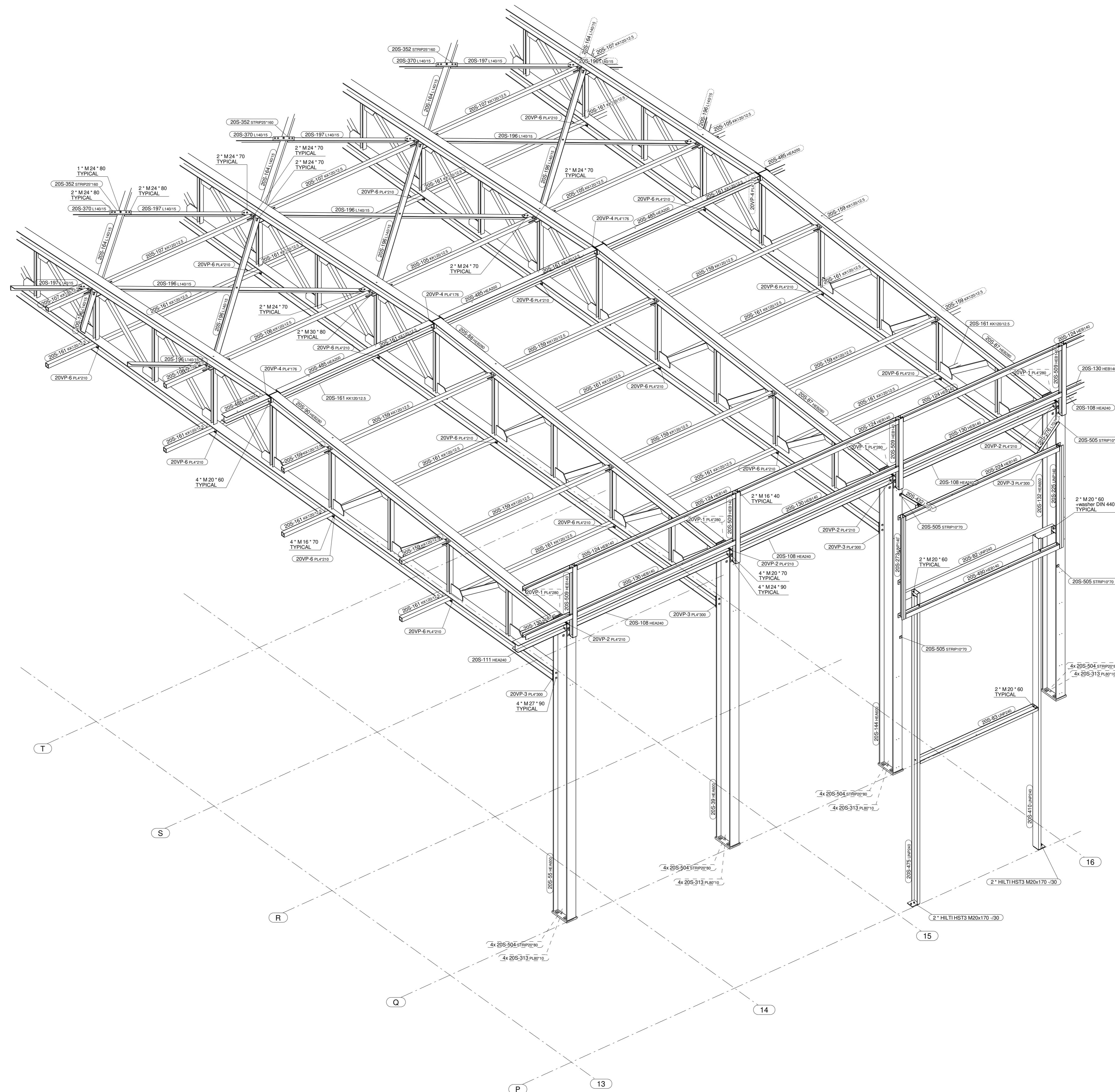
3D View - Low Hall - Grid 13-16 1:50
