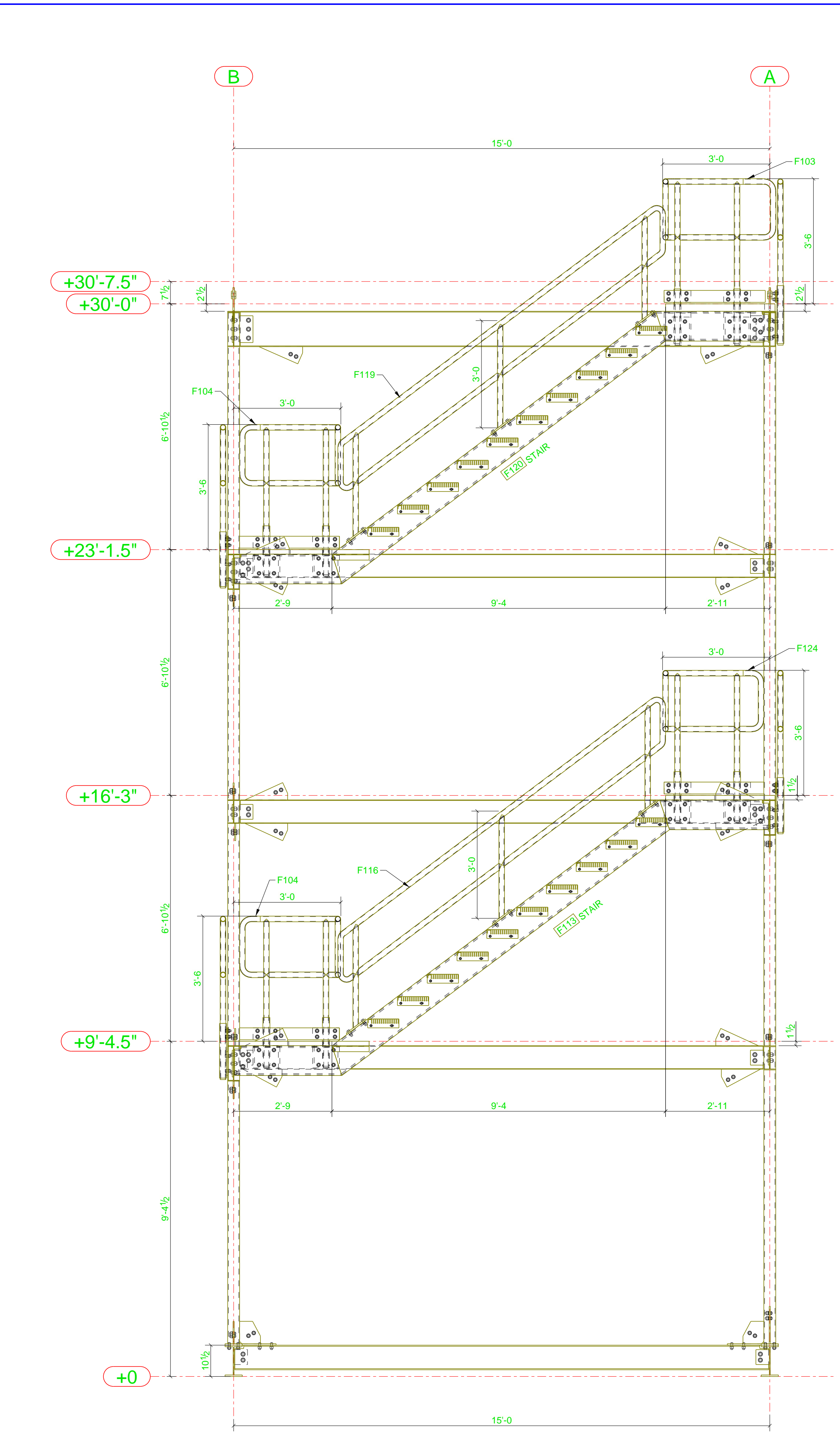
G ELEVATION G104 REF: E100
