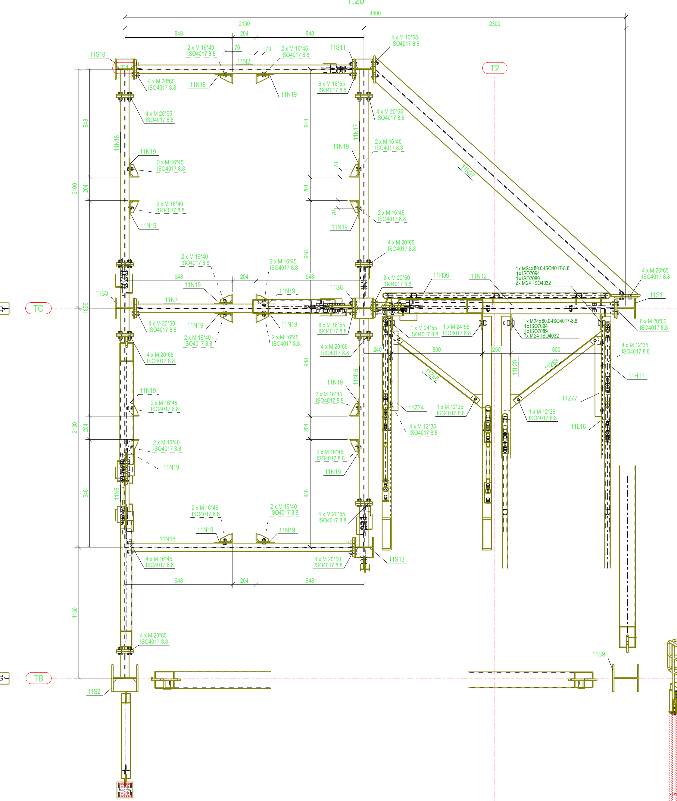
PLAN VIEW - TOWER +10.440 TOS
