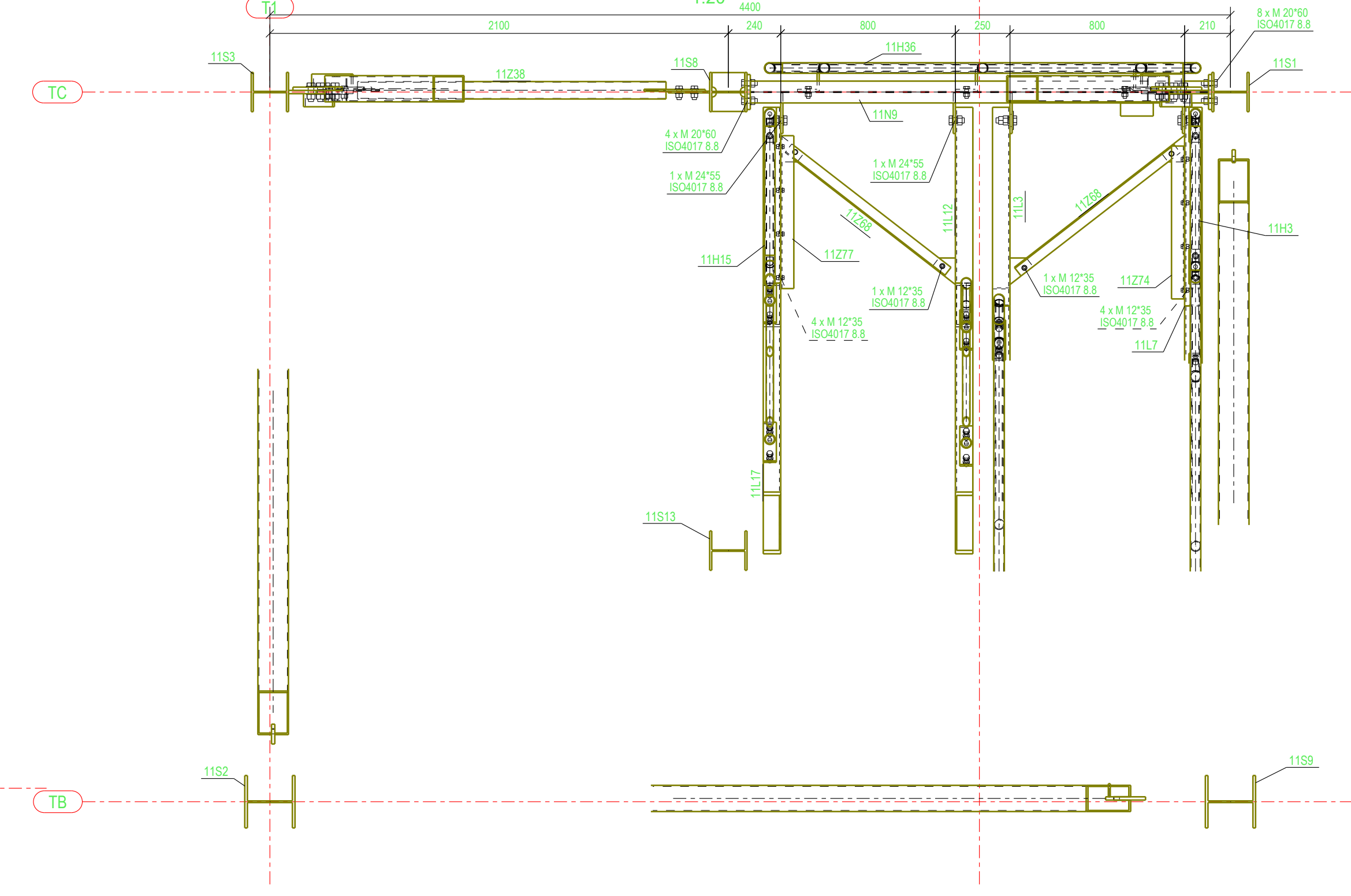
PLAN VIEW - TOWER +13.640 TOS
