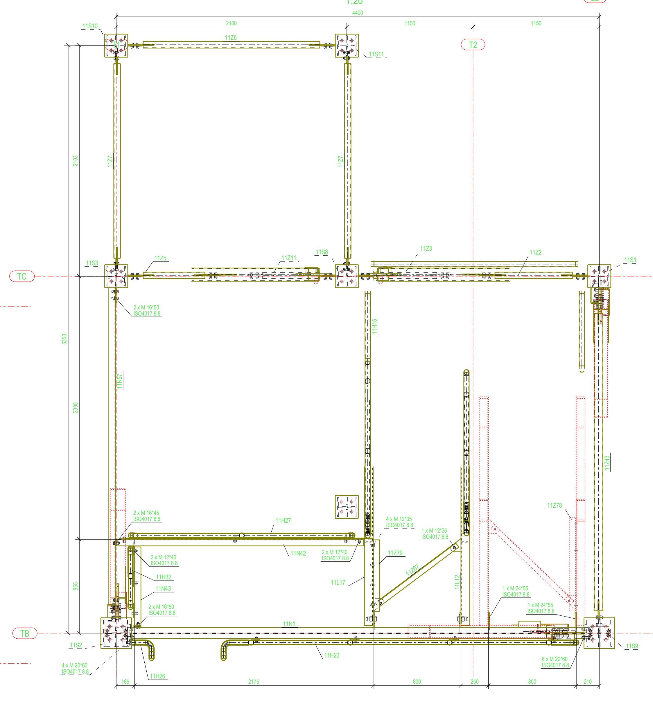
PLAN VIEW - TOWER +15.347 TOS
