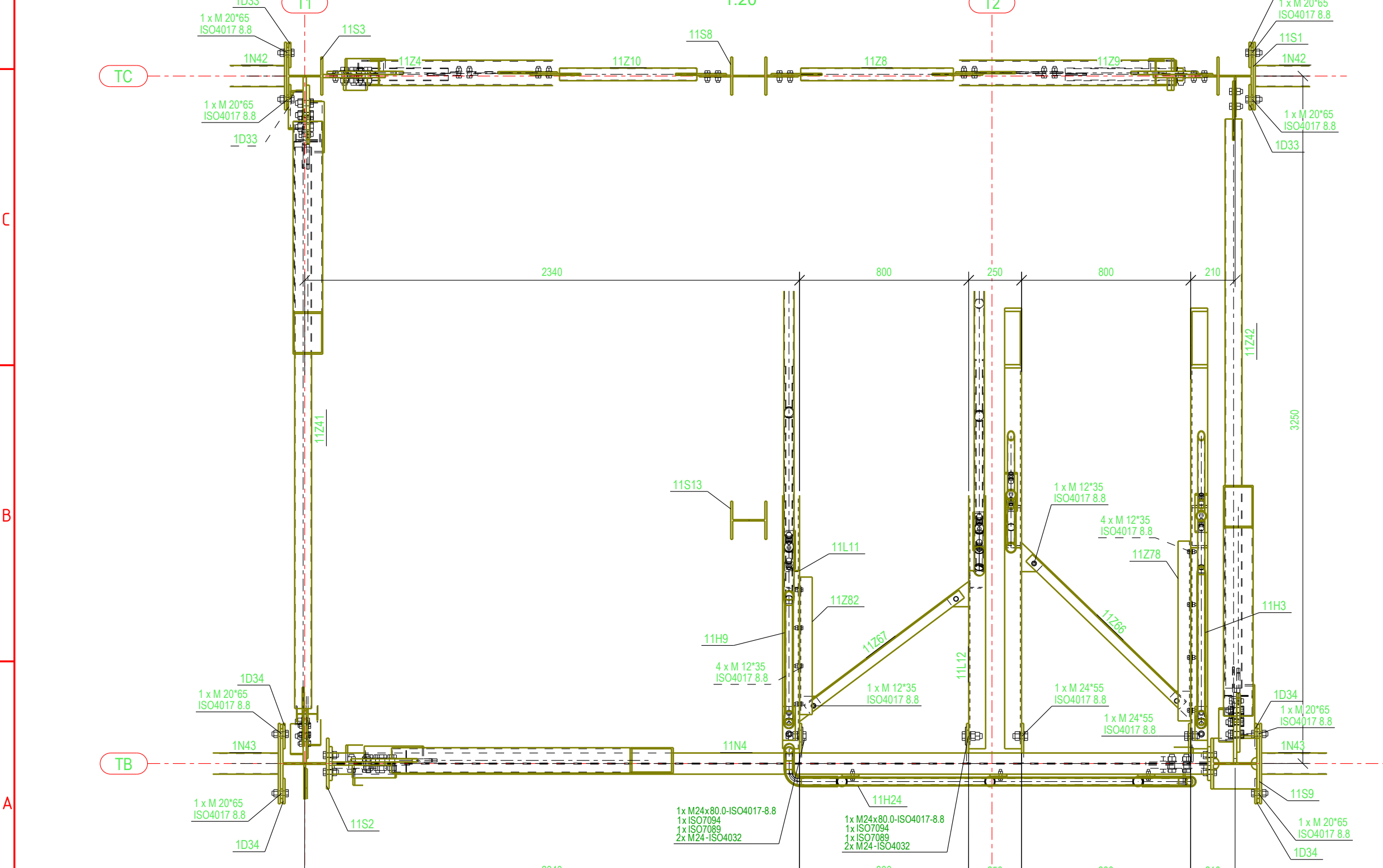
PLAN VIEW - TOWER +12.147 TOS
