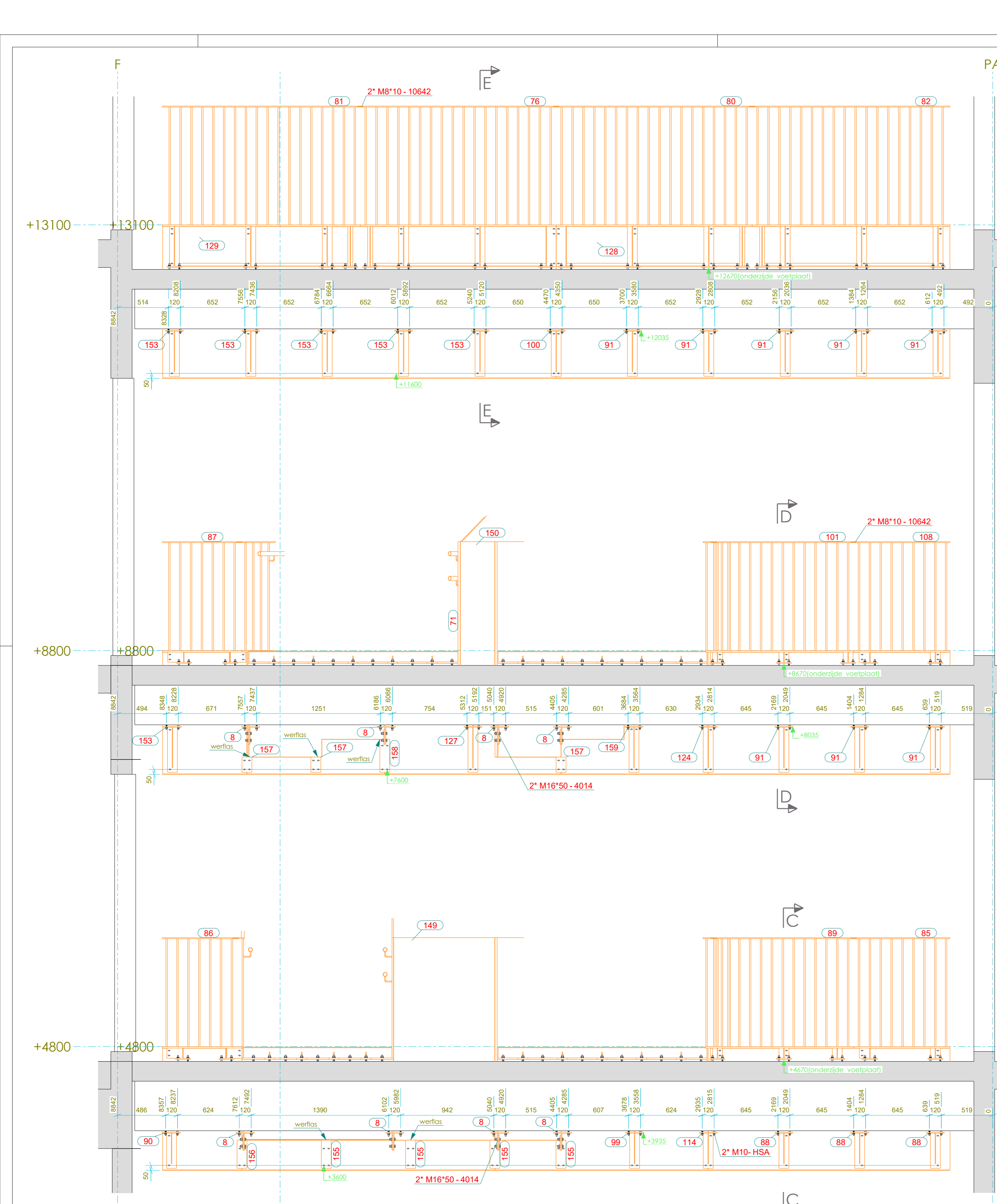
Snedes as P3 1:25
