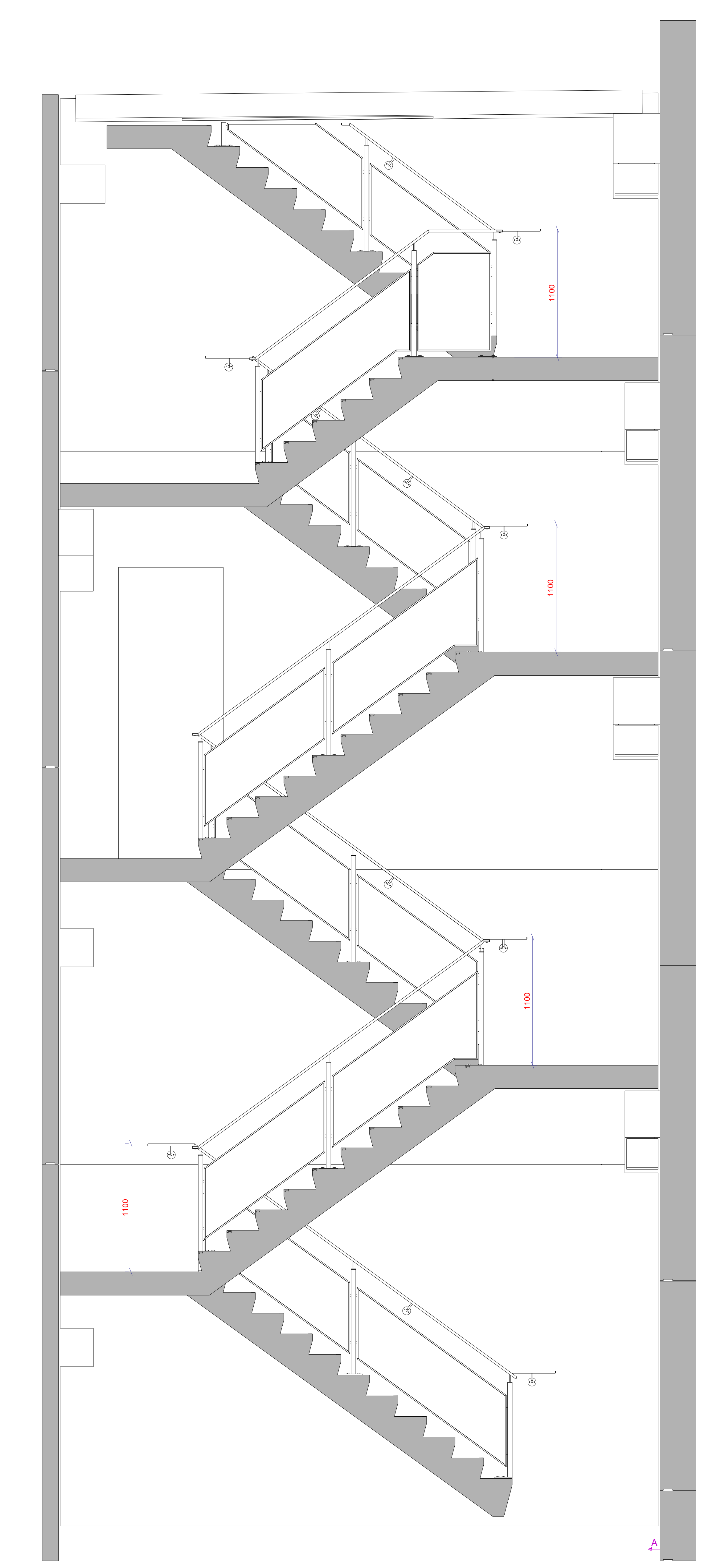
View_07 (3D) 1:20
