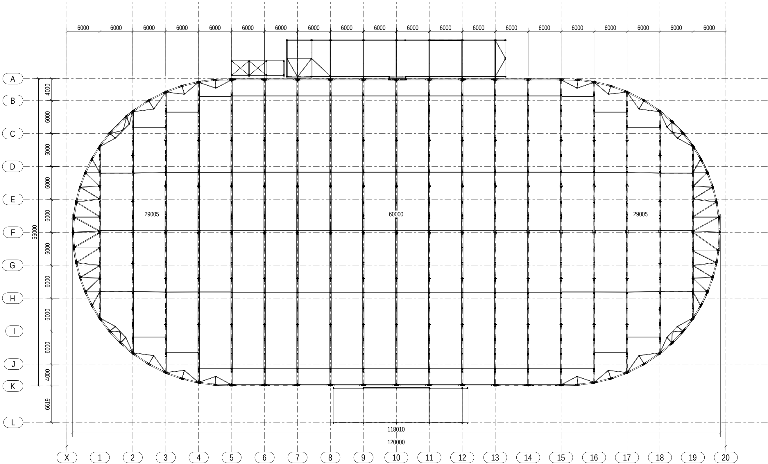
Top view outline
