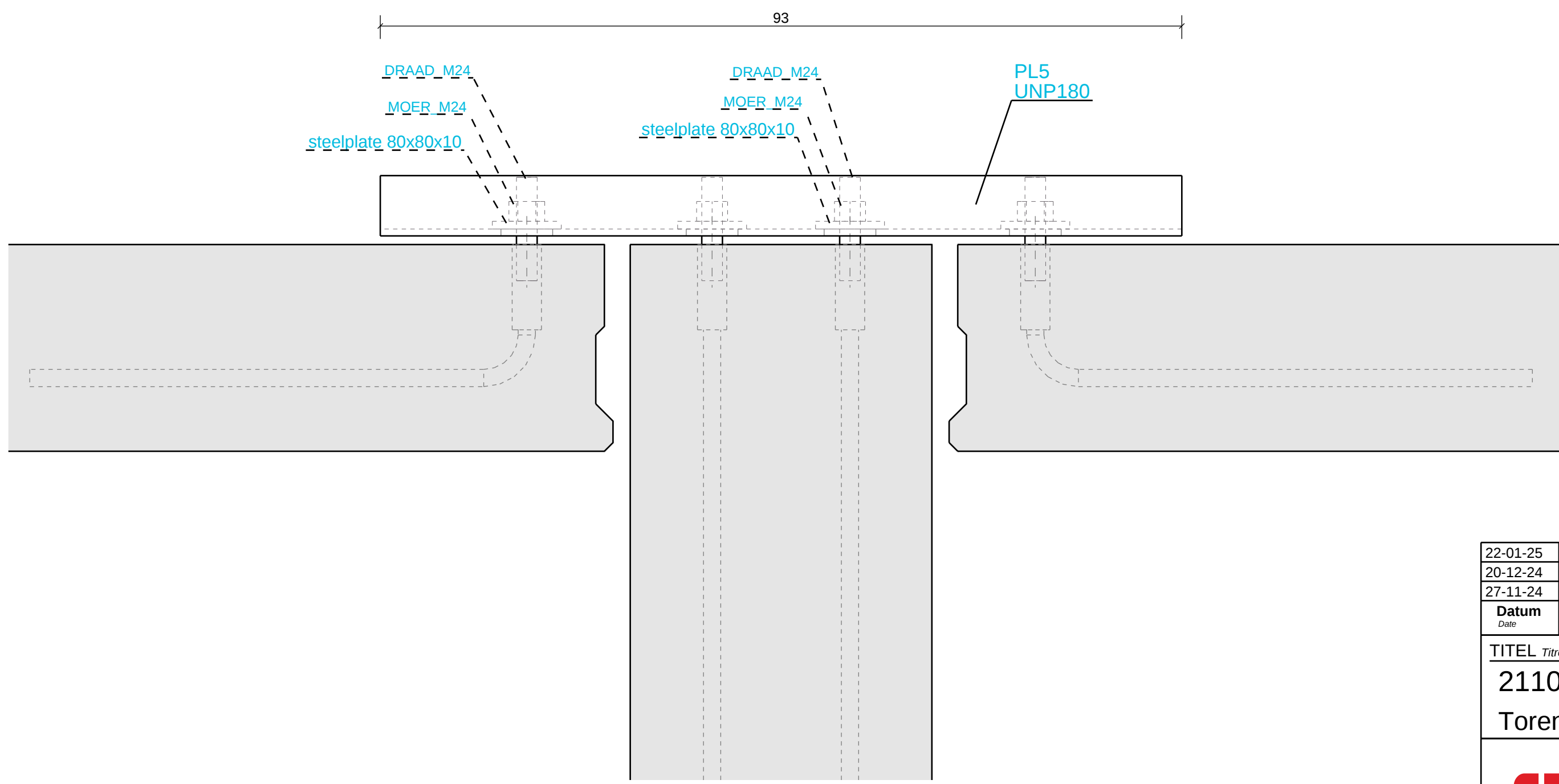
Typisch wand-vloer AS 13
