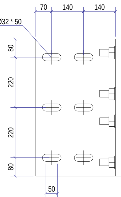
Detail D, 1:10
