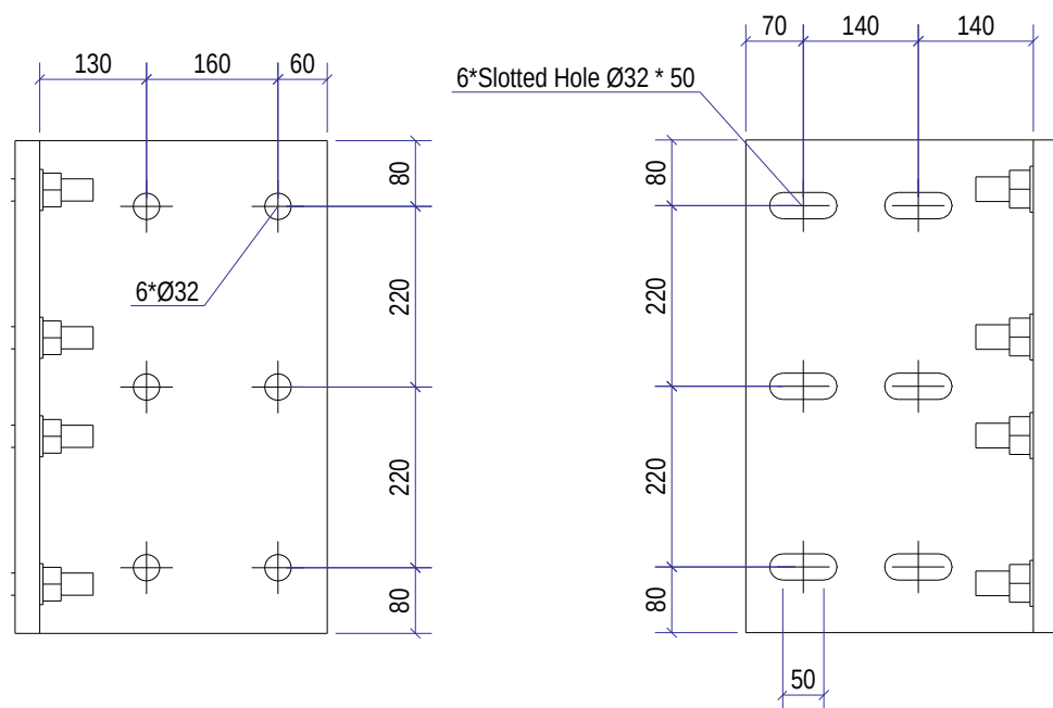
Detail B, 1:10
