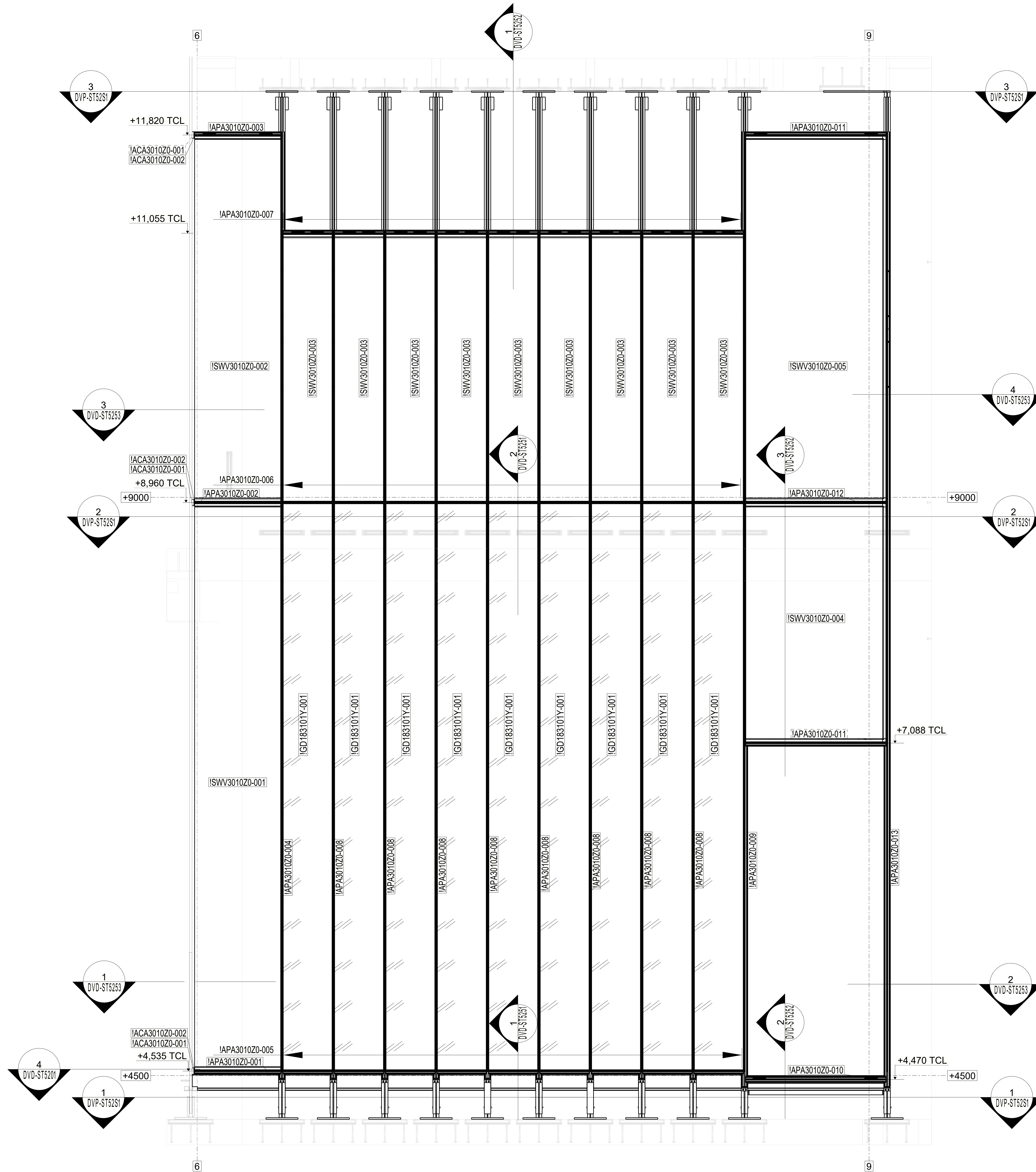
PARTIAL ELEVATION - SOUTH DVE-ST52S1 (L01-52)
