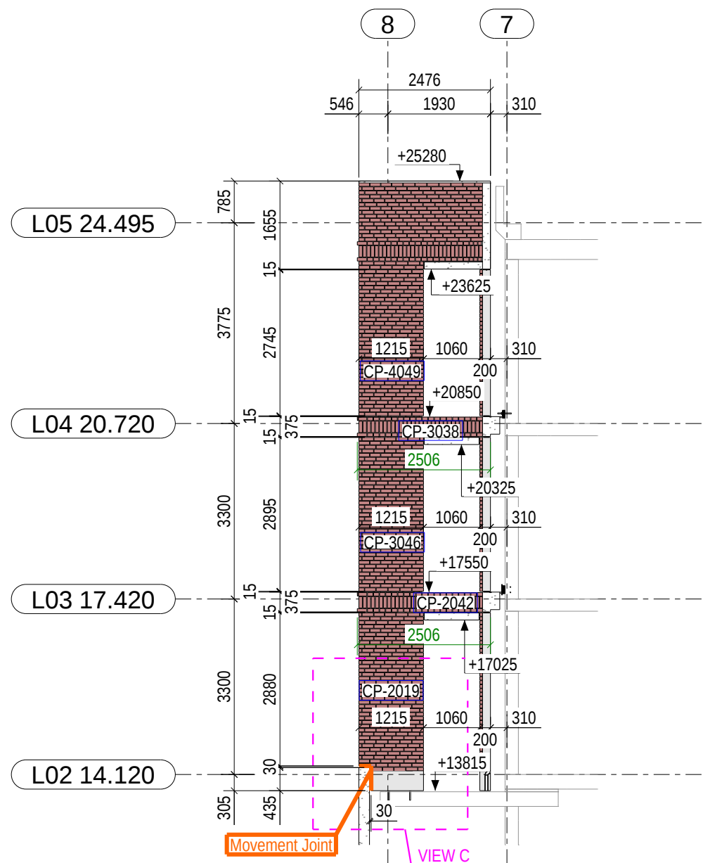
Set back elevation E (Makins Street Elevation) 1:100
