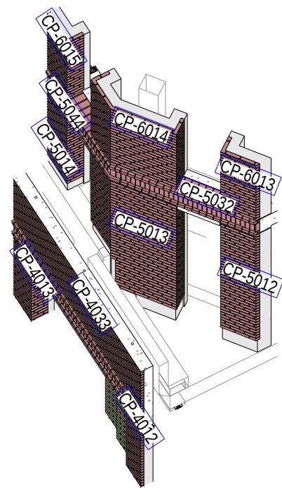
VIEW A - 3D VIEW 1:75
