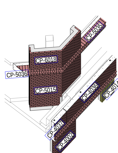
VIEW B - 3D VIEW 1:75
