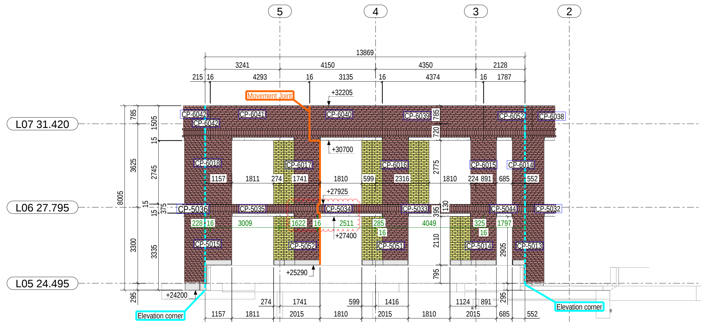
Set back 5th floor 1:100
