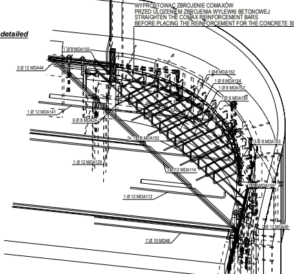
Corner in axis 1-E detailed 1:20
