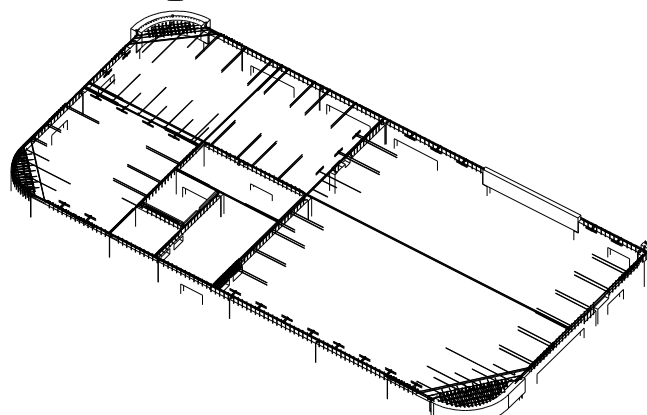
Joint reinforcement - 3D view 1:100
