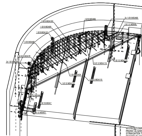
Corner in axis 1-A detailed 1:20
