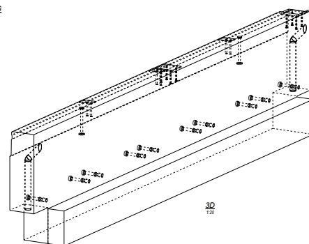
ARMERING 1:20
