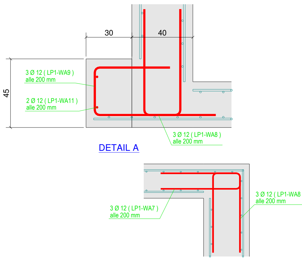
Detail hoekwapening
