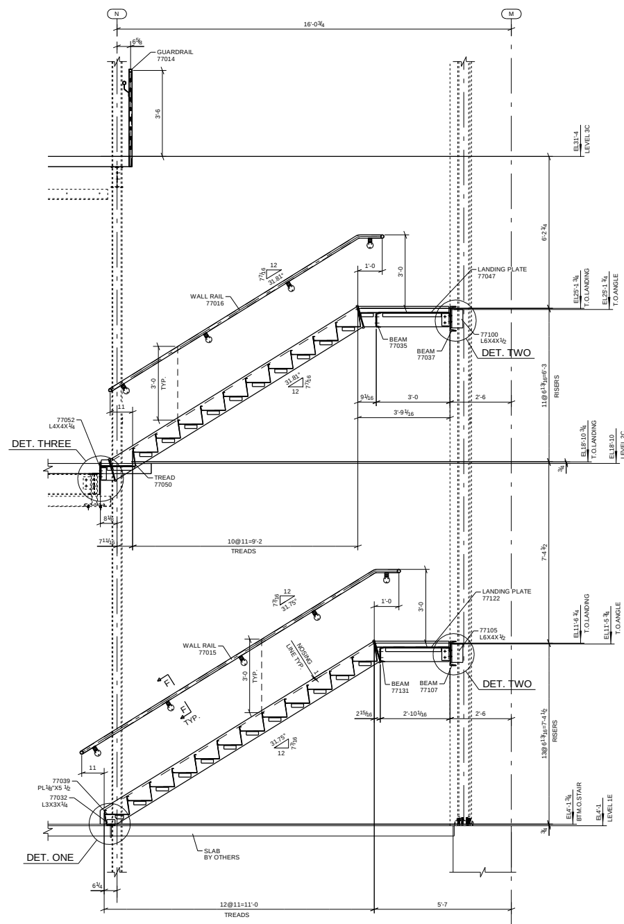
SECTION A - A (REF.: 4/ A6.02)
