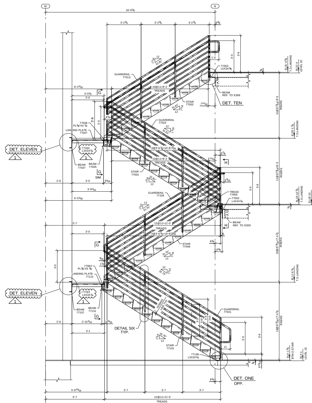
SECTION B - B (REF.: 4/ A6.02)
