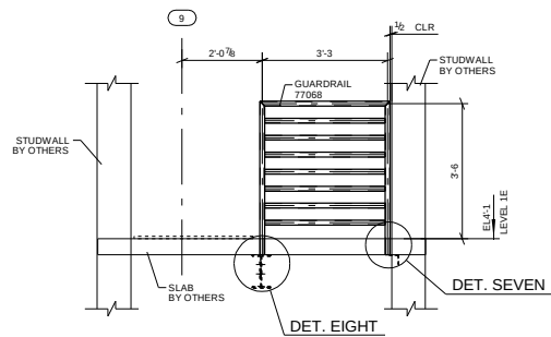
SECTION D - D (REF.: 4/ A6.02)
