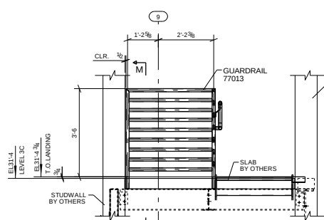
SECTION E - E (REF.: 4/ A6.02)
