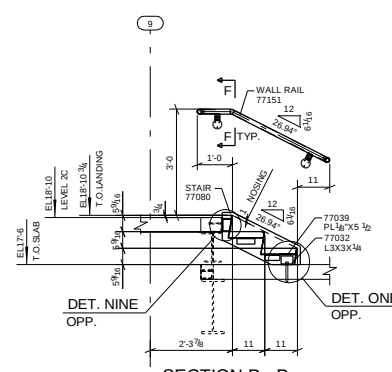
SECTION P - P (REF.: 4/ A6.02)
