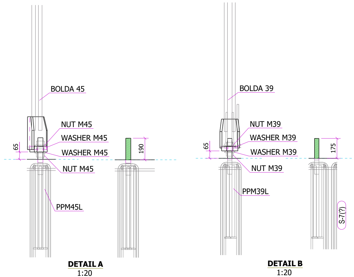
DETAIL FOR SUPPLEMENTARY REINFORCEMENT FOR PPM45L AND PPM39L 1:20
