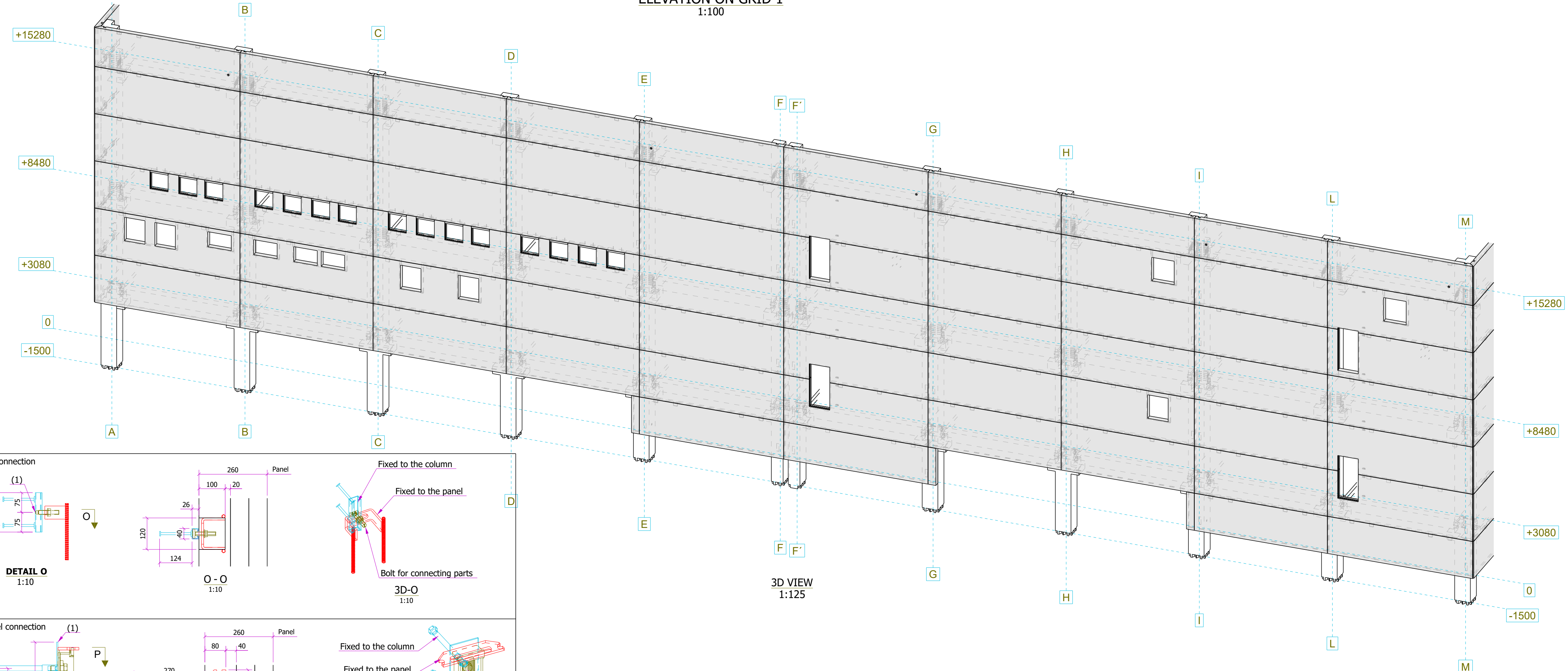
ELEVATION ON GRID 1 1:100
