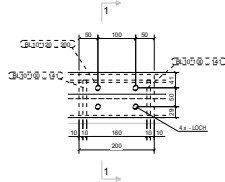
Detail A 1:5
