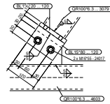
Detail C 1:5
