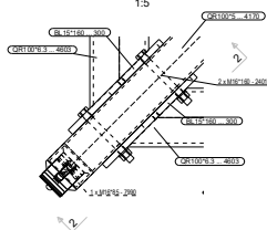
Detail B 1:5
