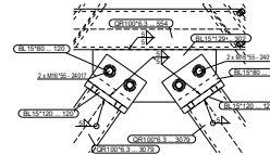
Detail D 1:5
