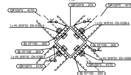
Detail E 1:5
